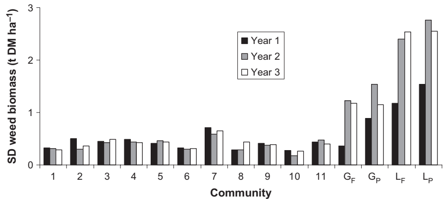
FIGURE 4 Standard deviation ( SD ) of annual weed biomass for a plot of each sown community for each of 3 years (estimate of within-site replicate variation aggregated over sites). Community 5 is the equiproportional community and G_F , G_P , L_F and L_P are the monocultures
