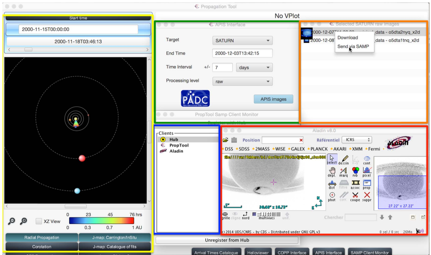
Fig. 4. Illustration of some VO functionalities available in the CDPP Propagation Tool. Yellow box: Location of the planets in the heliosphere (Earth in dark blue, Jupiter in red, Saturn in light blue) for the time period 15/11/2000-18/11/2000. Green box: APIS interface to query Hubble Space Telescope giant planet auroral observations using the EPN-TAP protocol. Orange box: results of the query. Blue box: SAMP client monitor activated. Red box: visualization in the Aladin tool of a giant planet auroral observation from the APIS database enabled by SAMP. (For interpretation of the references to color in this figure legend, the reader is referred to the web version of this article).
