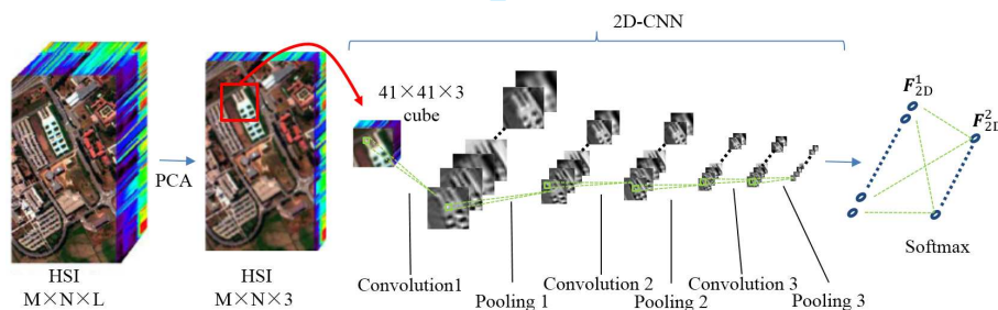
Figure 2. Illustration of 2D-CNN based spatial feature extraction framework.
