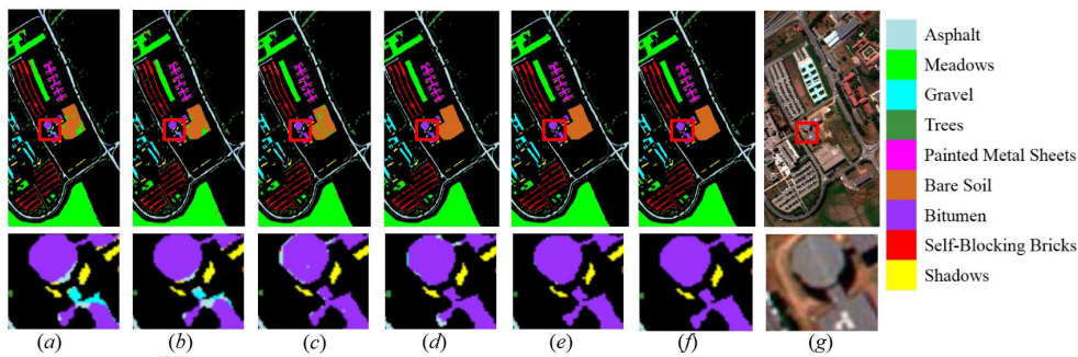
Figure 4. Classification results of Pavia University scene. (a) SSDCNN, OA=93.94%. (b) SSDL, OA=94.88%. (c) CNN, OA=96.57%. (d) DC-CNN, OA= 99.55%. (e) DC-CNN+ Augmentation , OA= 99.68%. (f) Ground truth. (g) False-color composite.
