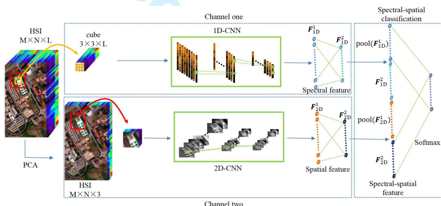
Figure 3. Illustration of DC-CNN based classification framework.
