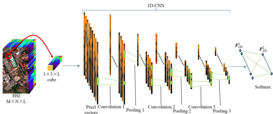
Figure 1. Illustration of 1D-CNN based spectral feature extraction framework.
