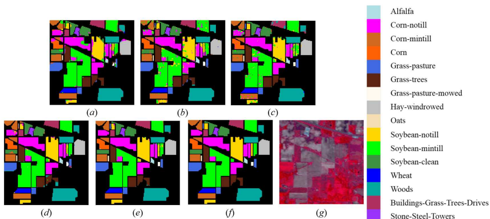
Figure 5. Classification results of Indian Pines scene. (a) SSDCNN, OA=90.76%. (b) SSDL, OA=91.60%. (c) CNN, OA=92.82%. (d) MD-CNN, OA= 96.88%. (e) MD-CNN+ Augmentation, OA= 98.76%. (f) Ground truth. (g) False-color composite.
