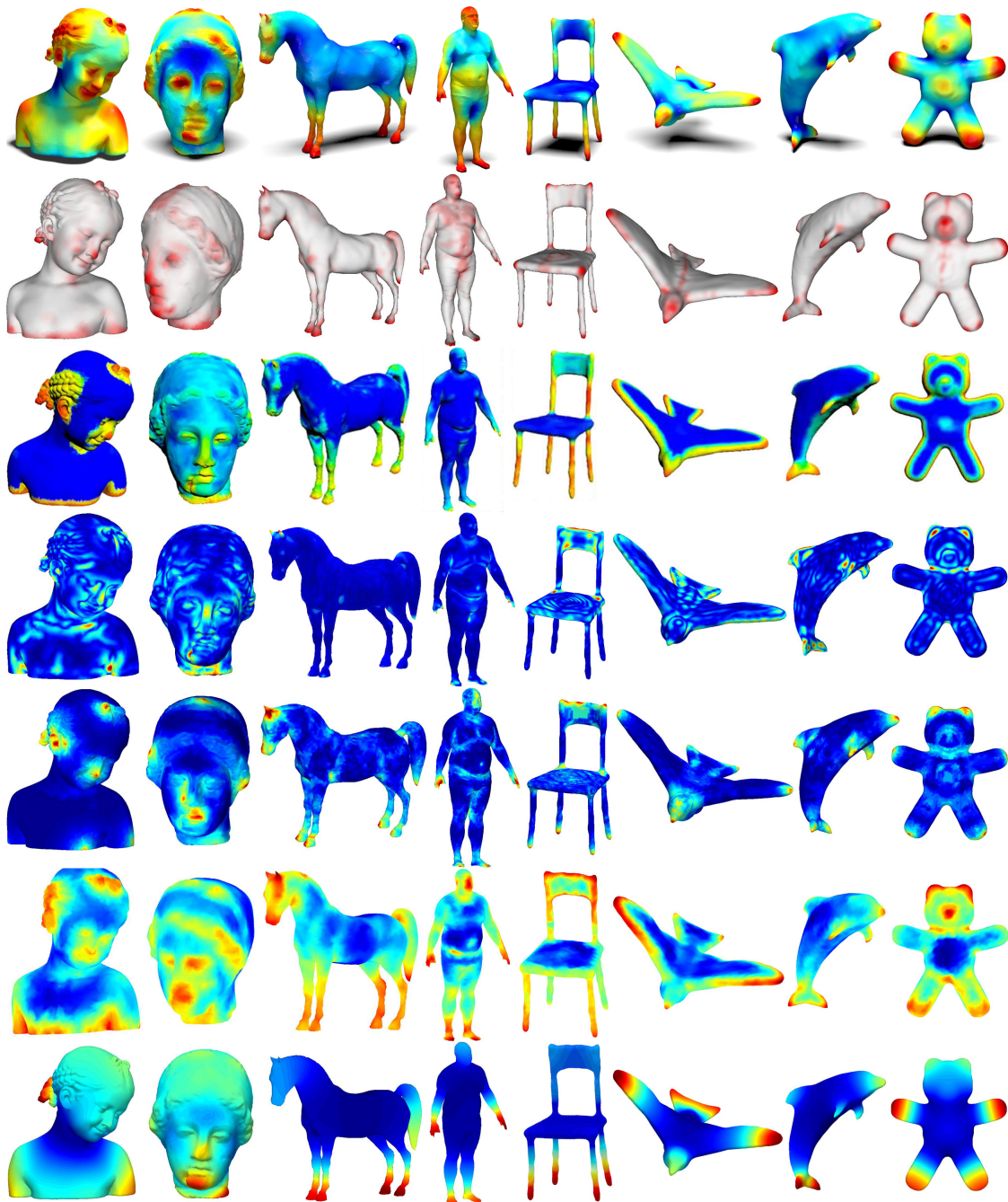
Fig. 8: Saliency detected by our method (first row) and the competing methods including (from the second row to the seventh row) [3], [32], [19], [21], [30] and [31]. Warm colors denote high saliency. These models are courtesy of the Watertight Models of SHREC 2007.
