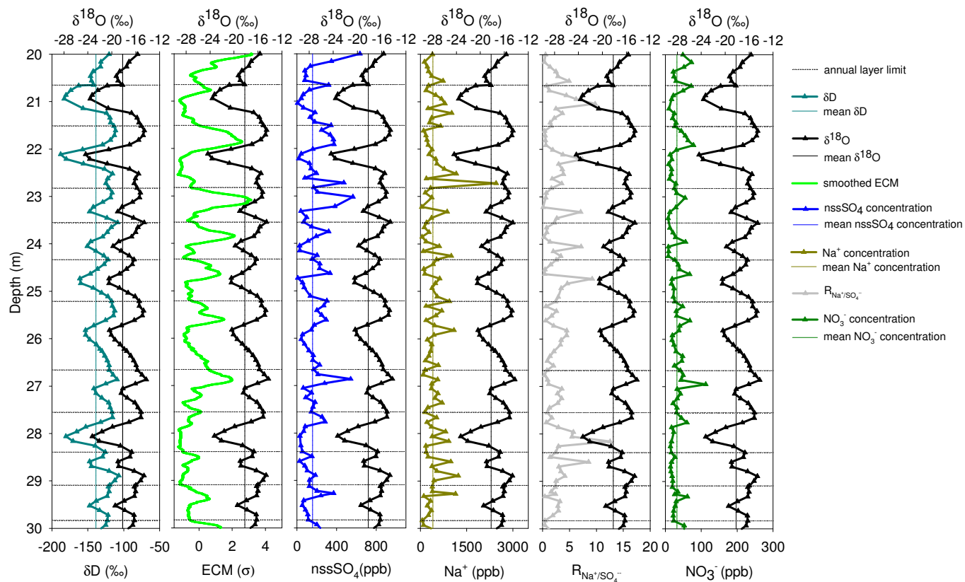
Figure 2. Variations in stable isotopes ( \delta^{18}O , \delta D ), smoothed ECM (running mean, 0.1 m), chemical species and their ratios used to constrain annual layer thickness in an example 10 m long section (20 - 30 m depth) of the IC12 ice core. Dashed horizontal lines indicate the annual layer limit (middle of the summer \delta^{18}O peak).
