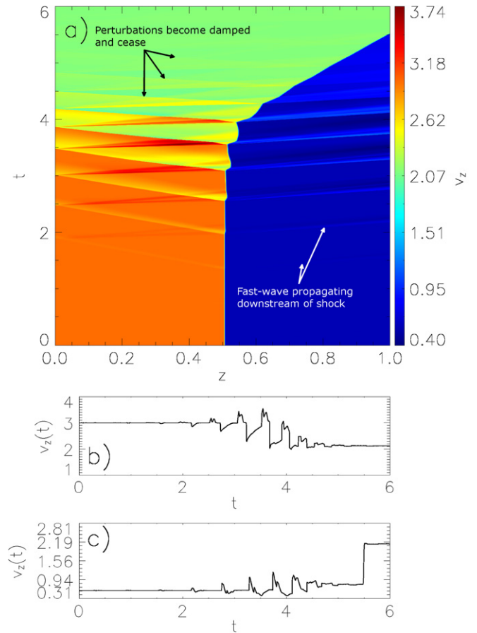
Figure 4. (a) Time–distance plot of the normalized longitudinal velocity, v_z . It can be seen that the gas-dynamic shock remains stationary until propagating fast shocks form. Here, the shock is impelled along the z -direction by each shock that “hits” the gas-dynamic shock. (b) The flow speed upstream of the shock ( z = 0.3 ) decreases as it is converted into twisting motions. Panel (c) shows the flow speed at z = 0.99 .
