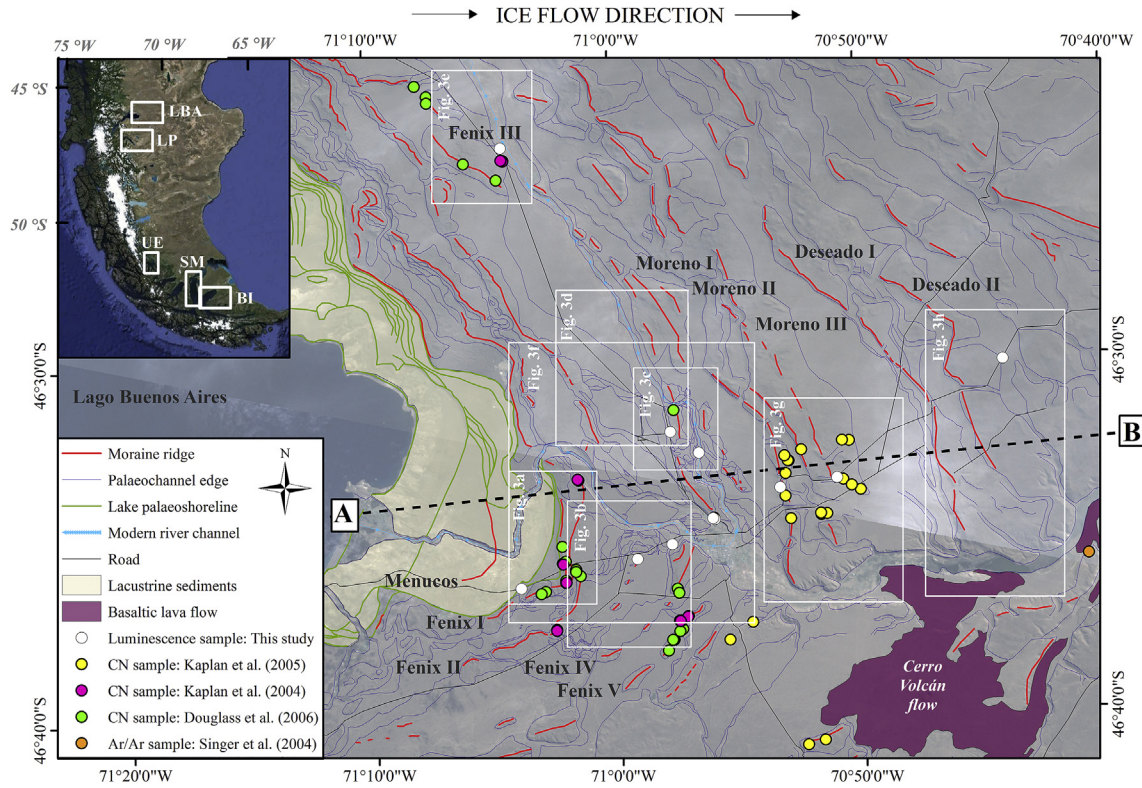
Fig. 1. Location of Lago Buenos Aires, Patagonia (GoogleEarth; Image © Landsat) and geomorphological map which includes the sites sampled for luminescence dating, the existing chronology and the locations of the images in Fig. 3. The inset shows the locations in South America of Lago Buenos Aires (LBA), Lago Pueyrredón (LP), the Última Esperanza region (UE), the Strait of Magellan (SM) and Bahía Inútil (BI).
