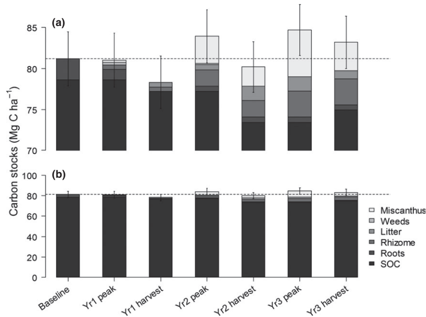
Fig. 10 Carbon stock assessments at peak yield (full senescence) and at spring harvest (following overwinter litter drop). Figures are presented in Mg ha -1 , Plot (a) shows a magnified image of individual pools (note y axis scales) while plot (b) shows the size of these gains and losses relative to the soil carbon pool and overall carbon stock. Error bars show standard errors propagated across all pools.
