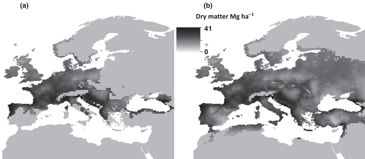
Fig. 2 A revised* crop yield prediction for M × g . Yield is displayed in grey scale from 41 (black) to 0 \text{Mg ha}^{-1} (Grey). The original M × g bioclimatic envelope (Hastings et al. , 2009a,b) is shown in (a) and the new estimation of the bioclimatic envelope for M × g and the new trialled hybrids is shown in (b) which is based on recent climate data 2000–2009 and FAO/IGBP plant available water estimates on a 5 min grid. The new cold limit considers the data from infield soil temperature measurements and the overwinter survival success. The new drought limit is based on observed infield drought responses and water balances with estimates of plant available water derived from depth and soil textures. This high-level analysis does not identify the marginal lands within the grids where the yields may be lower than those indicated. *Revised 2015, for the earlier version see Hastings et al. (2009a,b).
