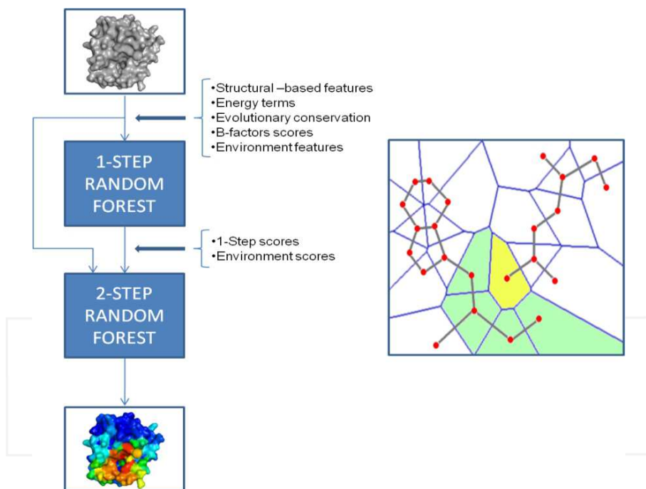
Fig. 2. Overview of prediction process in VORFFIP and a Voronoi Diagram of a interacting pair. The left side of the figure illustrates the 2-step prediction approach in VORFFIP. The right side of the figure shows the Voronoi Diagram of two neighbouring residues; heavy atoms are represented by red dots and coloured cells illustrate interaction between atoms of neighbouring residues.
