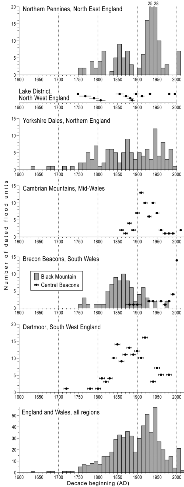
Figure 2. Decadal frequency of lichen-dated boulder-berms in upland areas of England and Wales. Where available (Dartmoor, Cambrian Mountains and Central Brecon Beacons) lichen dating accuracy is indicated by \pm 2\sigma error bars; for full details see Foulds et al., 2014a, 2014b and Matthews, 2015).
