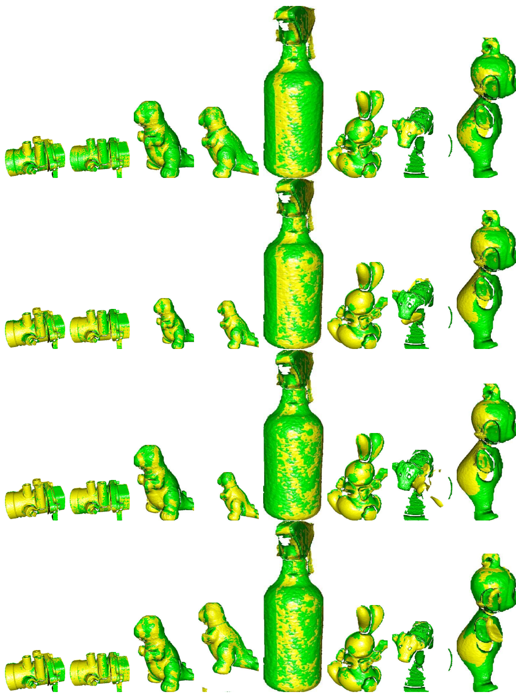
Figure 4: Registration results using the SoftICP algorithm for various shapes with key points selected from the data shape using different point selection algorithms. Rows, top to bottom: RKP, octave, MSFE, and NSS. Columns, left to right: valve20-10, valve10-0, dinosaur72-36, dinosaur36-0, bottle0-36, bunny80-60, cow49-45, and tubby120-80.
