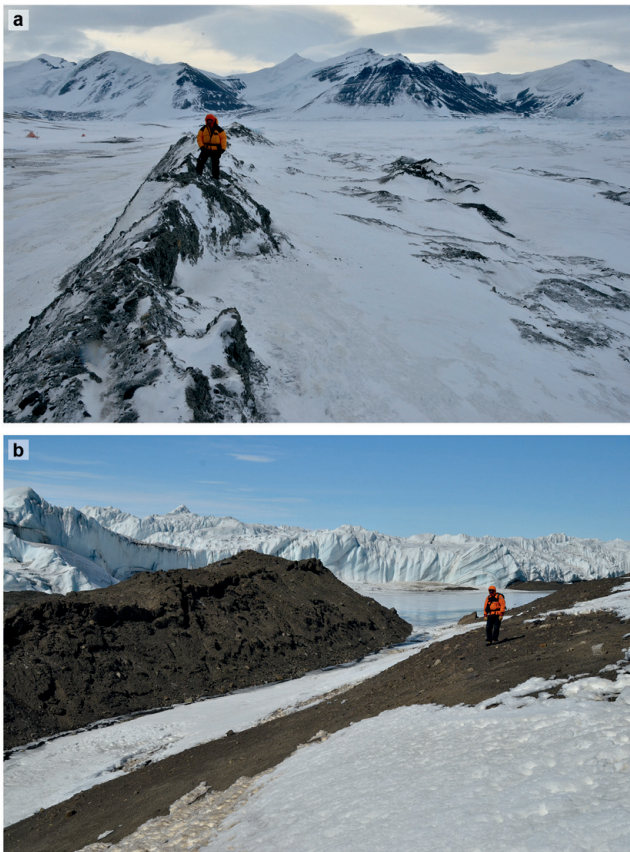
Fig. 6. Ice-shelf moraine morphology: (a) drape of diamicton overlying strongly foliated ice with minor debris near Ablation Lake; (b) ridge of sandy gravel at ice-shelf margin 500 m south of Moutonnée Lake.
