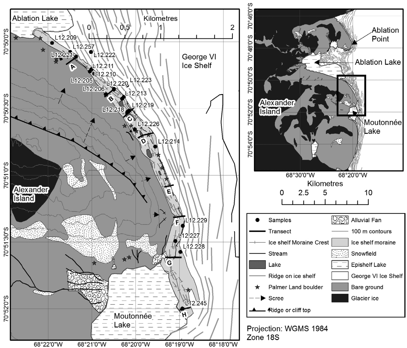
Fig. 4. Location of transects normal to the ice margin between Ablation Lake and Moutonnée Lake, and sediment locations in ice-shelf moraine.
