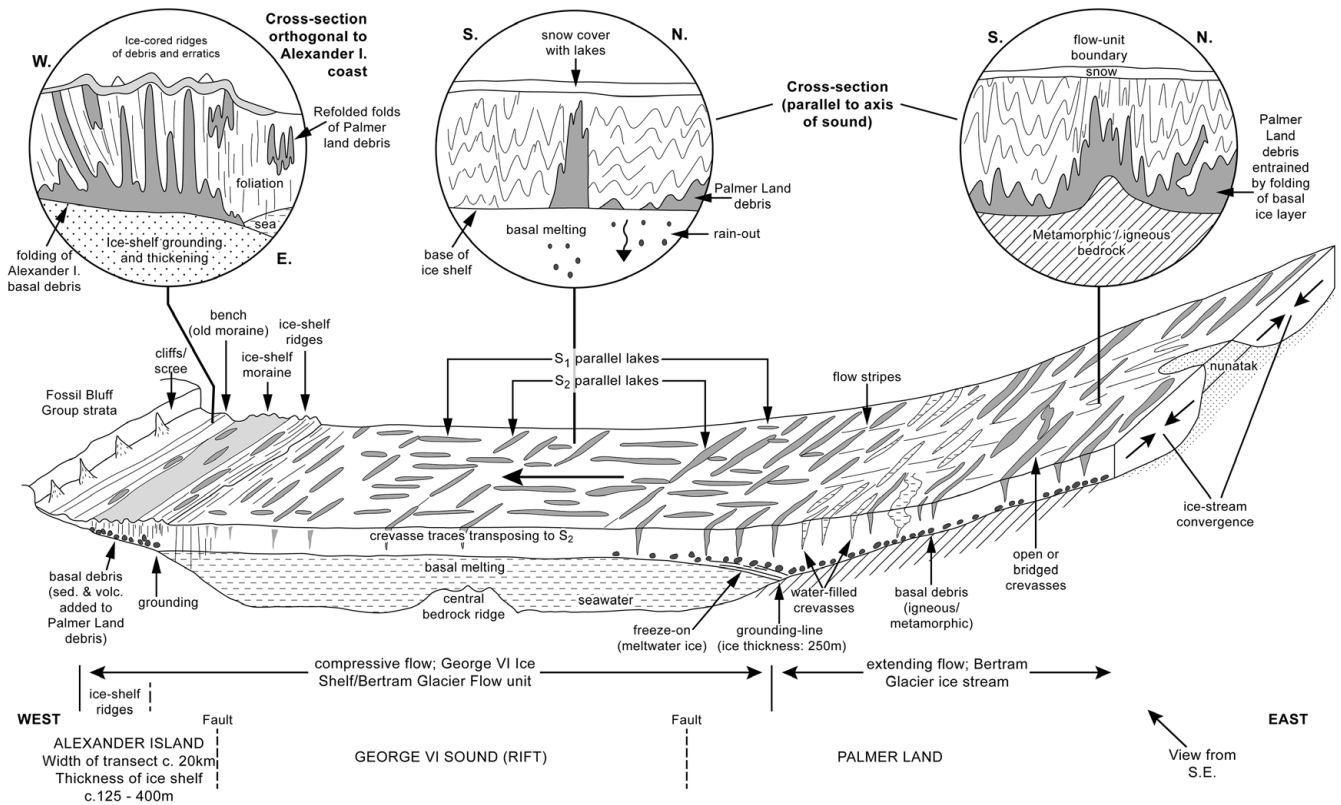
Fig. 11. Conceptual model of ice-shelf-moraine formation for George VI Ice Shelf, showing transition from grounded ice on Palmer Land to the floating ice-shelf reach, and its impingement on Alexander Island. Circles show details of inferred structural relationships.
