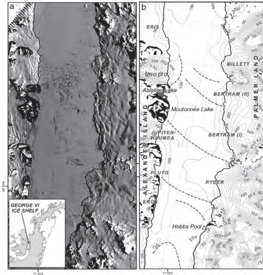
Fig. 1. The central part of George VI Ice Shelf, SW Antarctic Peninsula. (a) Landsat ETM+ 7 scene from 13 February 2003. The linear black areas on the ice shelf are structurally controlled surface lakes. (b) Ice-thickness data of ice shelf and source ice streams. Names refer to principal glacier flow-units.
