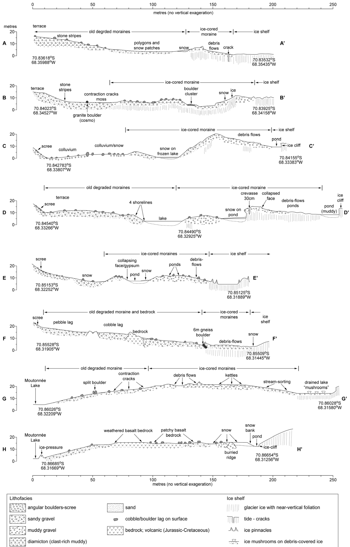
Fig. 5. Transects through ice-cored ice-shelf moraine indicating thickness and facies distribution (see Fig. 4 for location).
