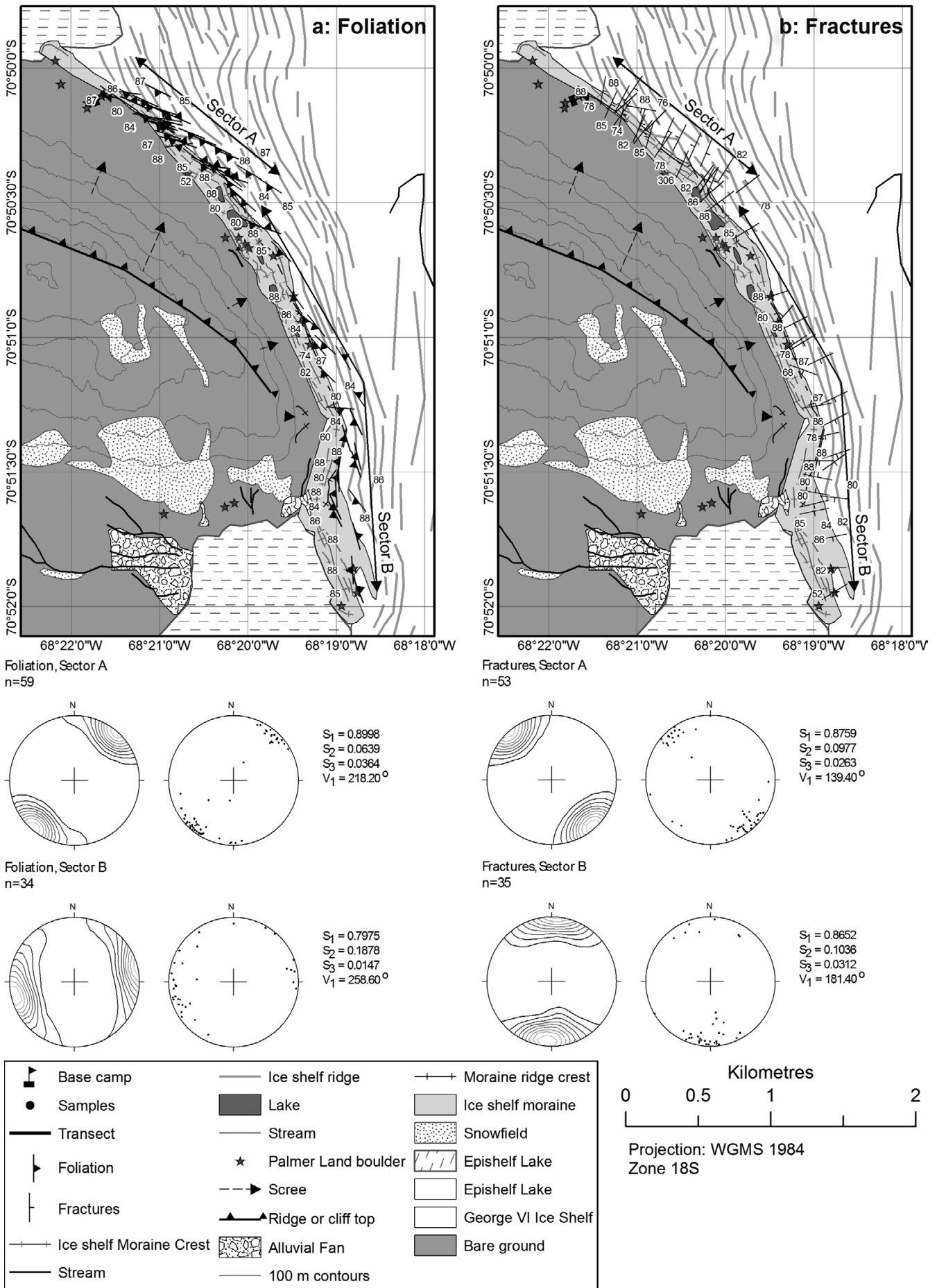
Fig. 7. Structural glaciological maps of zone between Ablation Lake and Moutonnée Lake, Alexander Island, showing (a) foliation and (b) fractures. Two sectors of uniform foliation orientation are defined, with accompanying stereographic (lower hemisphere, equal-angle) projections for each sector and each structure, together with eigenvalues.
