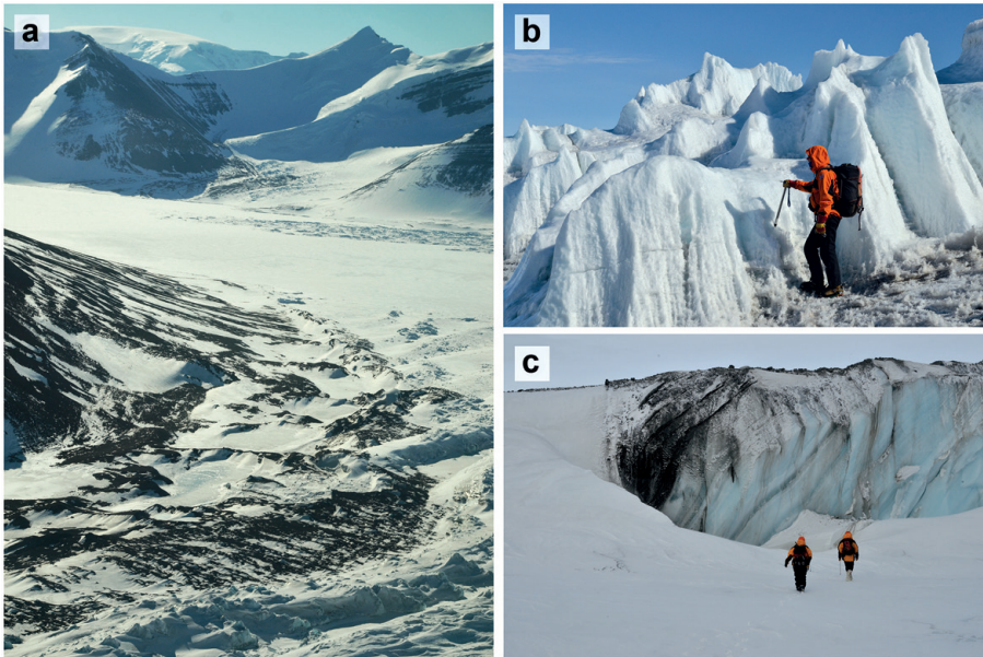
Fig. 3. Ice-shelf morphology. (a) Overview of ice-shelf moraines and Ablation Lake from the air; (b) pinnacles and 'ice ships' whose morphology is controlled by foliation and differential weathering; (c) debris layers forming ice-shelf moraine in ice cliff between Ablation Lake and Moutonnée Lake.
