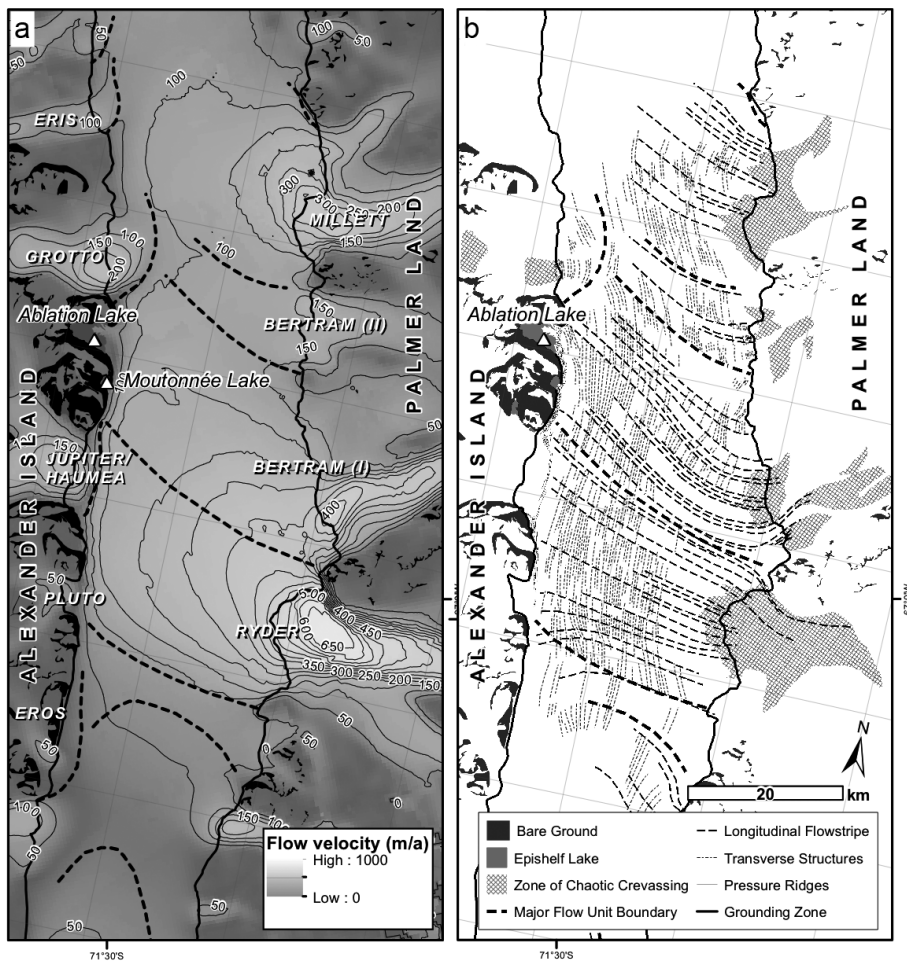
Fig. 2. Dynamics and structure of central George VI Ice Shelf. (a) InSAR-derived velocity distribution (Rignot et al. 2011). (b) Structural map of longitudinal structures (foliation) and transverse structures (crevasse traces, transposing to coast-parallel foliation), and flow-unit boundaries, based on the distribution of elongated lakes.
