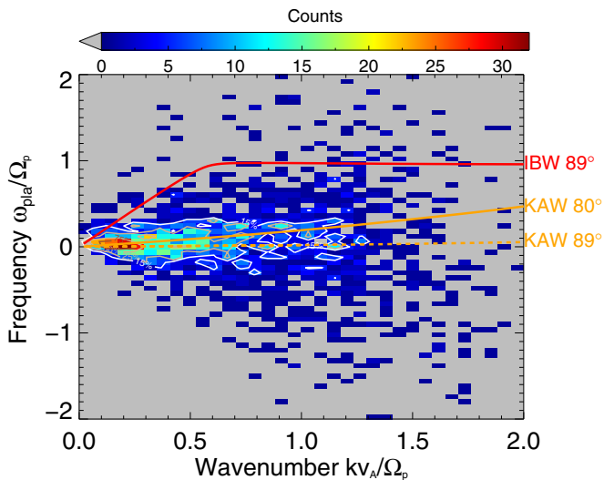
Figure 3. Two-dimensional histogram with the dispersion points from all 52 intervals with curves from linear Vlasov solver of Li & Habbal (2001) for ion Bernstein at \theta_{\mathbf{kB}} = 89^\circ and kinetic Alfvén waves at \theta_{\mathbf{kB}} = 80^\circ and 89^\circ .
