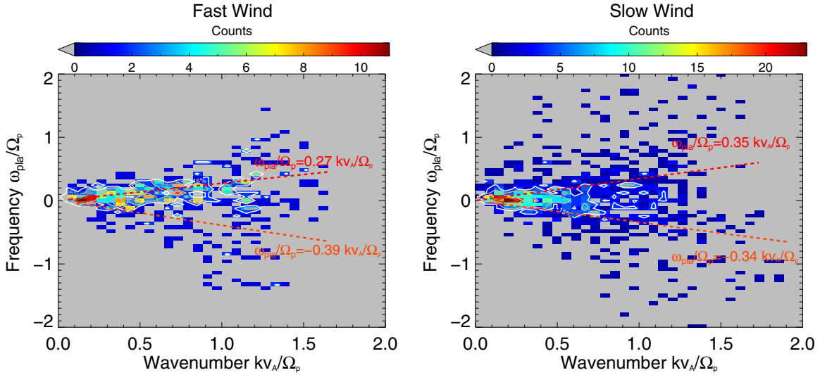
Figure 4. Two dimensional histogram with bins of 0.06 \times 0.06 made up of only fast solar wind (11 intervals) cases V_{sw} > 540 \text{ km s}^{-1} (left) and only (41 intervals) slow solar wind cases V_{sw} < 470 \text{ km s}^{-1} . The red (orange) dashed line denotes a linear least squares fitting to the data for positive (negative) points.
