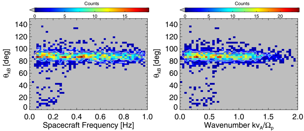
Figure 2. Plots of the angle that the wavevector at the maximum value of P(\omega, \mathbf{k}) makes with the global mean magnetic field \mathbf{B}_0 as a function of spacecraft frequency (left) and wavenumber (right). The contours denote to 15% (dark brown), 25% (light brown), 50% (white), and 75% (dark red) of the maximum counts. The coding of contours will be the same in all of the figures.
