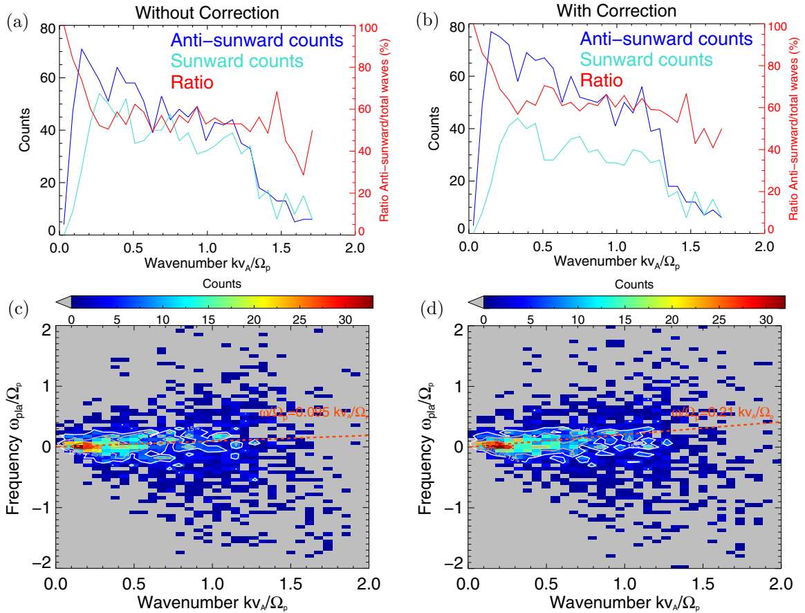
Figure 5. Top row: counts of negative (sunward) and positive (anti-sunward) waves as a function of the wavenumber obtained from k -filtering without the correction (a) and with (b). Bottom row: dispersion plots of all intervals without (c) and with (d) the corrections. A linear least squares fitting is shown in the orange dashed lines to quantify the effect of the correction.
