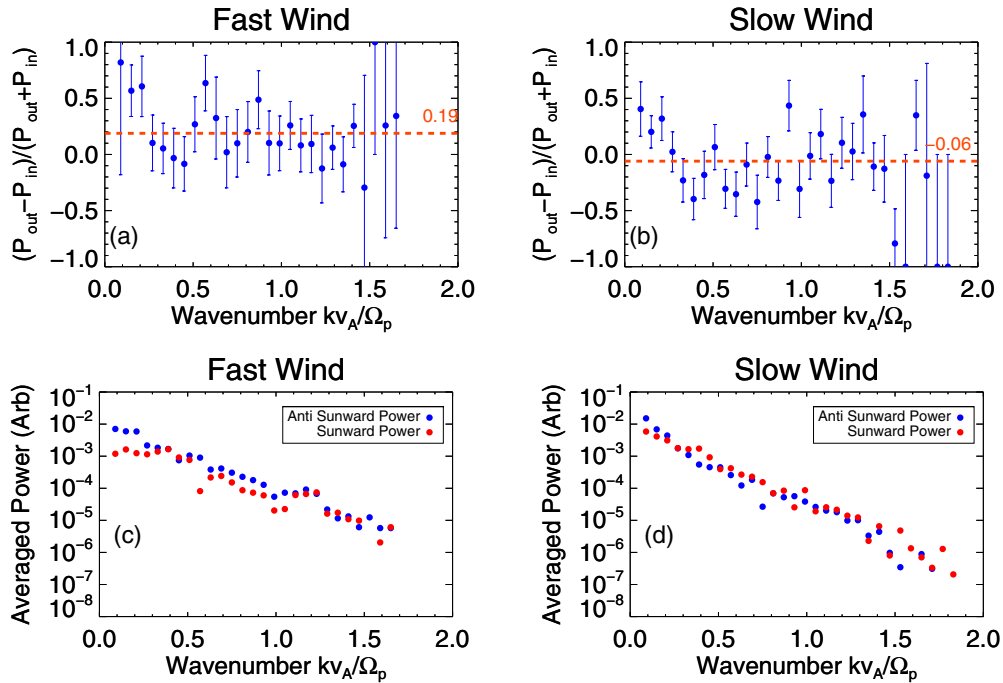
Figure 6. (a and b) shows the ratios of the powers (P_{\text{out}} - P_{\text{in}})/(P_{\text{out}} + P_{\text{in}}) , where +1 denotes all power being anti-sunward and -1 denotes all power being sunward, as a function of wavenumber for fast and slow cases. The orange dashed lines denote the weighted average of (P_{\text{out}} - P_{\text{in}})/(P_{\text{out}} + P_{\text{in}}) . (c) and (d) show the evolution of the total sunward and anti-sunward power as a function of wavenumber bin.
