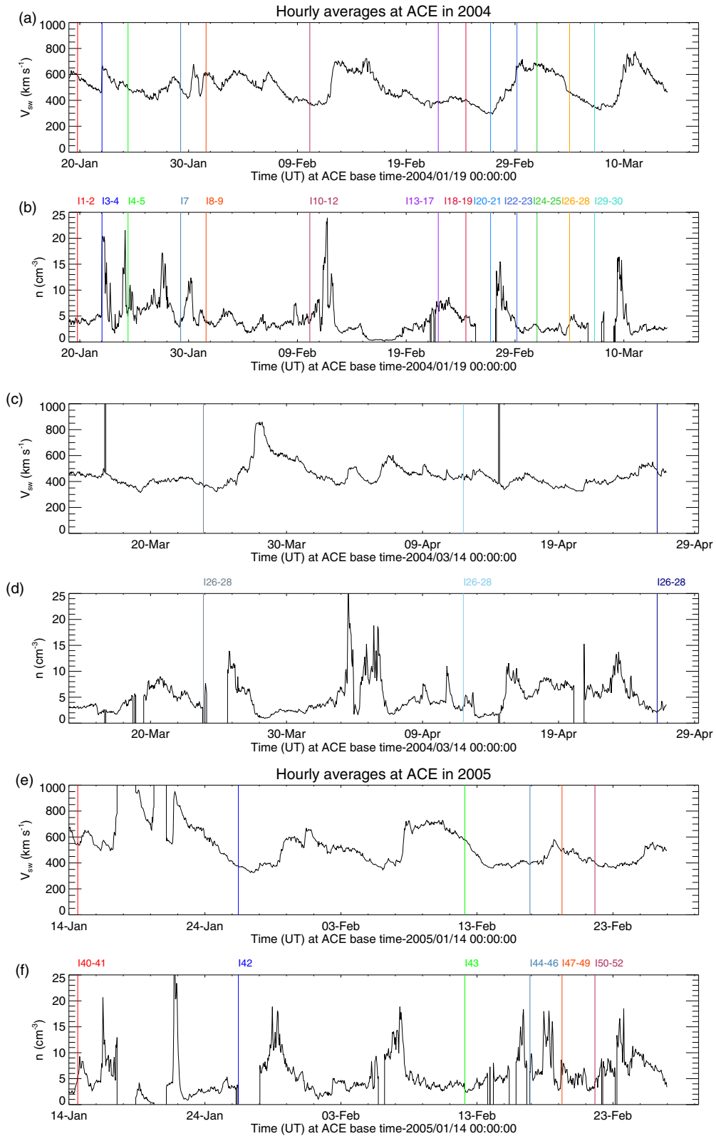
Figure 1. Panels (a), (c), and (e) show the hourly averages of the radial velocity of the solar wind at the L1 Lagrange point measured by ACE in 2004 (a and c) and 2005 (e). Panels (b), (d), and (f) show the corresponding hourly averages of number density of protons. Missing data are denoted by large positive (velocity) and negative (density) values and lie out of the plotting range
