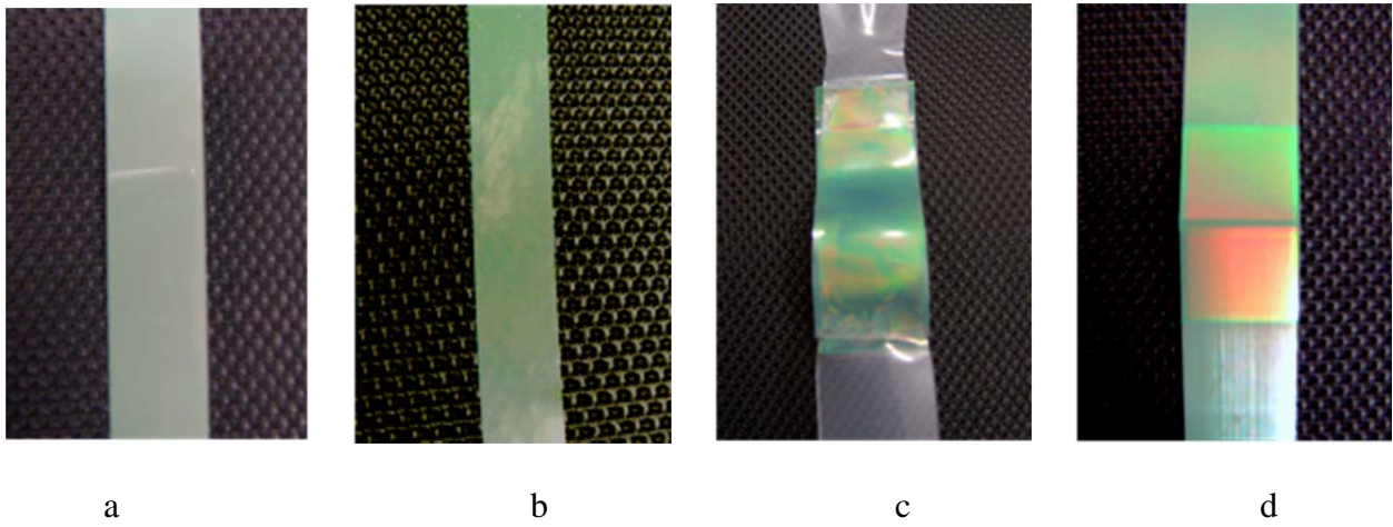
Figure 5. Representative photographs showing optical appearance of polymer opal samples. a) Initial tape. b) Tape after MPR tensile deformation. c) Tape after MPR simple shear deformation. d) Tape after successive MPR edge-shearing deformation.
