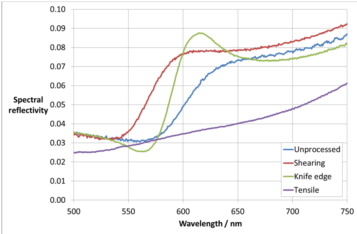
Figure 6, Representative spectra on the variation of polymer opal outer surface spectral reflectivity as a function of wavelength for different types of deformation applied to the tape for; MPR unprocessed tape, MPR simple shear V=0.5\text{mm/s} , MPR tensile test V=0.5\text{mm/s} and MPR edge shearing. MPR processed , V= 1\text{mm/s} . T=100\text{ }^{\circ}\text{C} for all experiments
