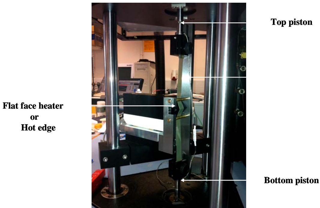
Strata Technology “edge shearing” MPR fitting
