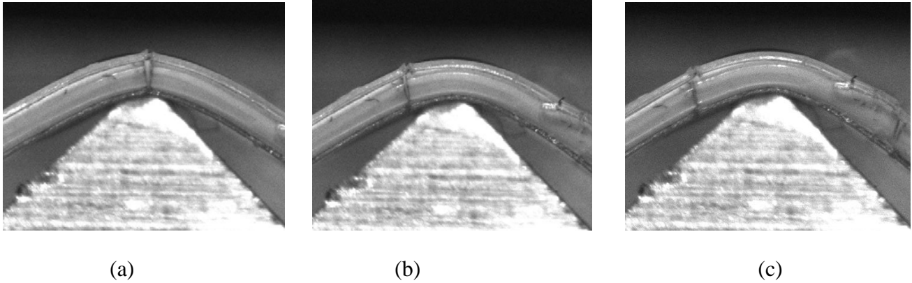
Figure 8. Side view photographic sequence of Polymer Opal sample being edge sheared from right to left, (a)-(c). T=25^{\circ}\text{C} . Piston tape translation velocity= 1mm/s. Approximate thickness of sample = 0.5mm The photograph shows the V metal edge and the foam, sandwiched between a top and bottom PET tape. The vertical marker line shown in 7a is seen to shear as the sample progressively moves from right to left over the edge as shown in figures 7b and 7c
