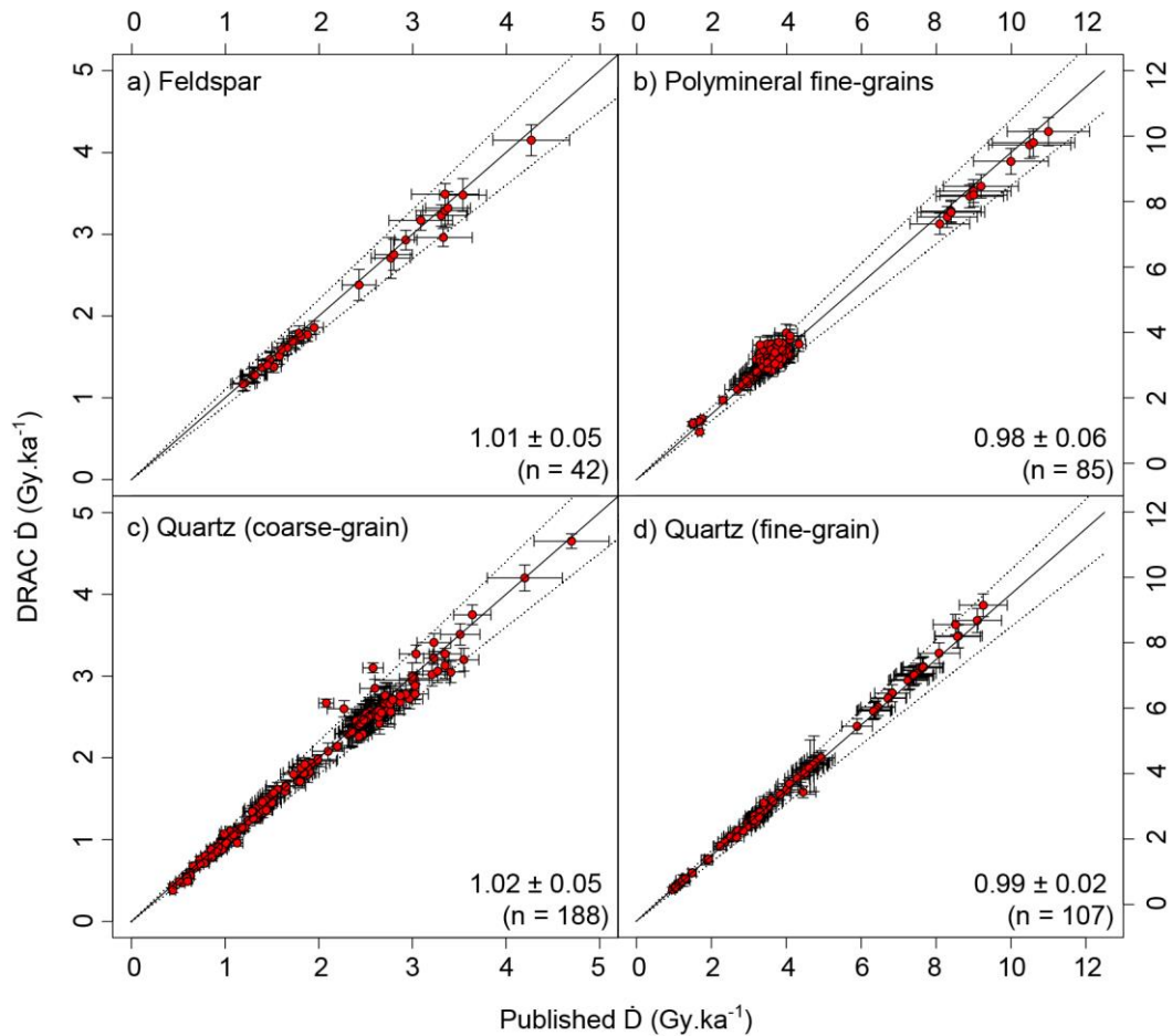
Figure 5: Comparison of dose rates ( \dot{D} ) calculated in DRAC with those previously published. Data are plotted separately for a) feldspar, b) polymineral, c) coarse-grain ( >63 \mu\text{m} ) quartz and d) fine-grain ( <63 \mu\text{m} ) quartz. 422 samples from 32 studies are compared with a mean ratio of 1.01 \pm 0.05 . If not stated in the publication, the following parameters were used to facilitate comparison: conversion factors – Adamiec and Aitken (1998), no Rb calculation from K, grain size attenuation for \dot{D}_\alpha and \dot{D}_\beta – Bell (1980) and Mejdahl (1979) respectively, etch depth – 9 \mu\text{m} , etch depth attenuation – Bell, 1979, a-value either 0.086 \pm 0.0043 , 0.035 \pm 0.001 (Rees-Jones and Tite, 1997) or 0.15 \pm 0.015 (Balescu and Lamothe, 1994) dependent on mineral and grain-size, overburden density – 2.0 \pm 0.1 \text{ g.cm}^{-3} , latitude, longitude and altitude estimated from Google Earth. The studies used for the DRAC comparison: Alappat et al., 2011, Bates et al., 2003, Breman et al., 2003, Buylaert et al., 2007 and Clark-Balzan et al., 2012, Davidovich et al., 2012, Demeter et al., 2012, Fuchs et al., 2012, Haberzettl et al., 2009, Halfen et al., 2010, Hall et al., 2010, Houben et al., 2013, Kaiser et al., 2009, Kars et al., 2012, Kels et al., 2014, Klasen et al., 2011, Kock et al., 2009, Kreutzer et al., 2012, Le Dortz et al., 2009, Lepper et al., 2013, Lomax et al., 2014, Madsen et al., 2009, Roskosch et al., 2012, Schatz et al., 2012, Schmidt et al., 2014, Schokker et al., 2005 and Stevens et al., 2011, Tamura et al., 2011, Thiel et al., 2011, Xu et al., 2010 and Yang et al., 2010.
