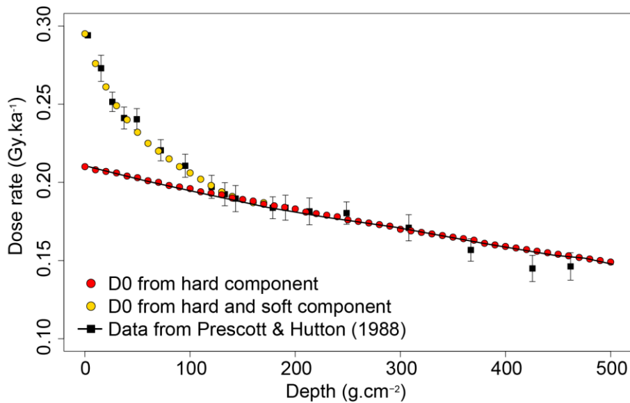
Figure 4: Penetration depths of cosmic rays. The original data from Barbouti and Rastin (1983) as presented in Prescott and Hutton (1988) are shown, together with their fit for the hard component. Data fitted for this study for the contributions from both soft and hard components (depths < 167 \text{ g.cm}^{-2} ) and from hard components only (depths > 167 \text{ g.cm}^{-2} ) are shown.
