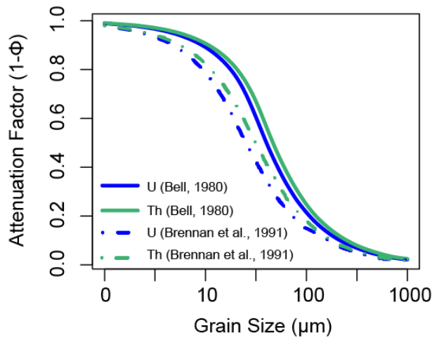
Figure 2: Grain size attenuation factors for \hat{D}_\alpha , interpolated from the original data of Bell (1980) and Brennan et al. (1991) using a spline fit. The original and fitted data are available in Tables S3.3a and S3.3b.
