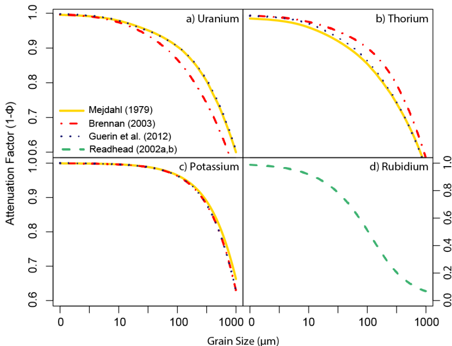
Figure 3: Grain size attenuation factors for \hat{D}_\beta , interpolated from the original data of Mejdahl, 1979, Brennan, 2003 and Guerin et al., 2012 and Readhead, 2002a and Readhead, 2002b. Note that only the quartz factors of Guerin et al. (2012) are shown, but both the quartz and feldspar factors are available for use within DRAC. The original and fitted data are available in Tables S3.4a and S3.4b.
