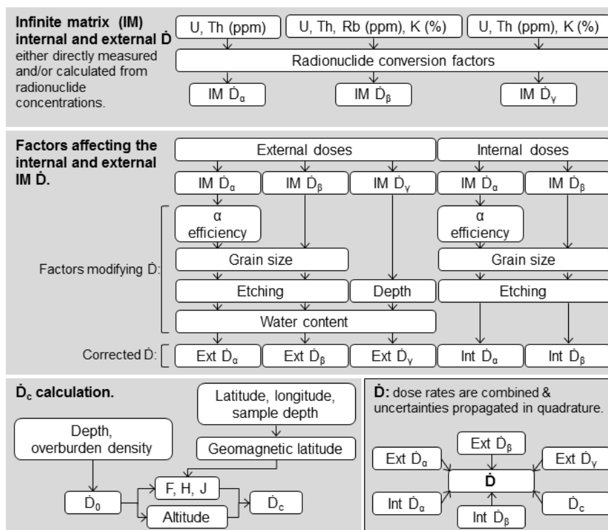
Figure 1: Overview of the \dot{D} calculation for trapped charge dating applications. IM – infinite matrix, ext – external, int – internal.
