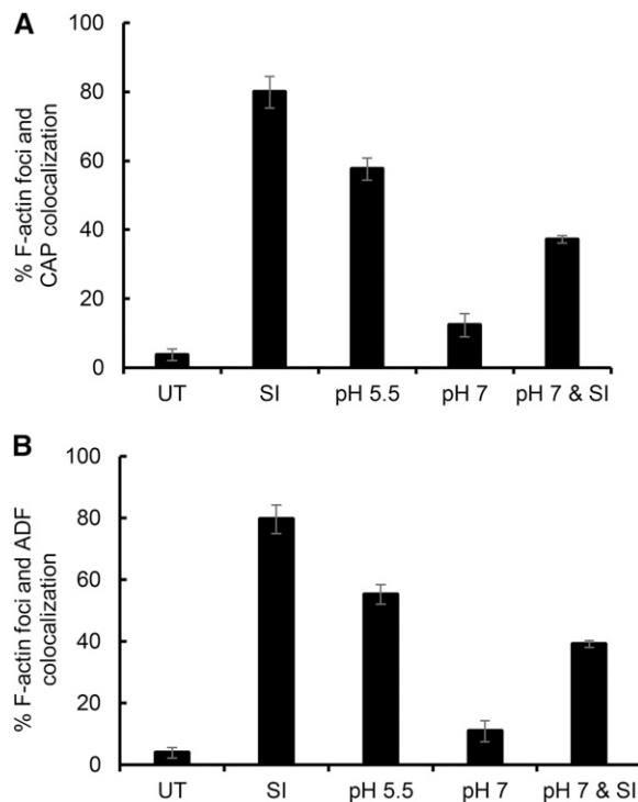
Figure 4. Acidification of the pollen tube cytosol triggers the formation of punctate F-actin foci and colocalization of CAP and ADF. A, Quantification of F-actin and CAP colocalization. Pollen tubes were scored for actin foci and CAP colocalization in three independent experiments ( n = 700 per treatment over three independent repeats). B, Quantification of F-actin and ADF colocalization. Pollen tubes were scored for actin foci and ADF colocalization in three independent experiments ( n = 700 per treatment over three independent repeats). UT, Untreated.
