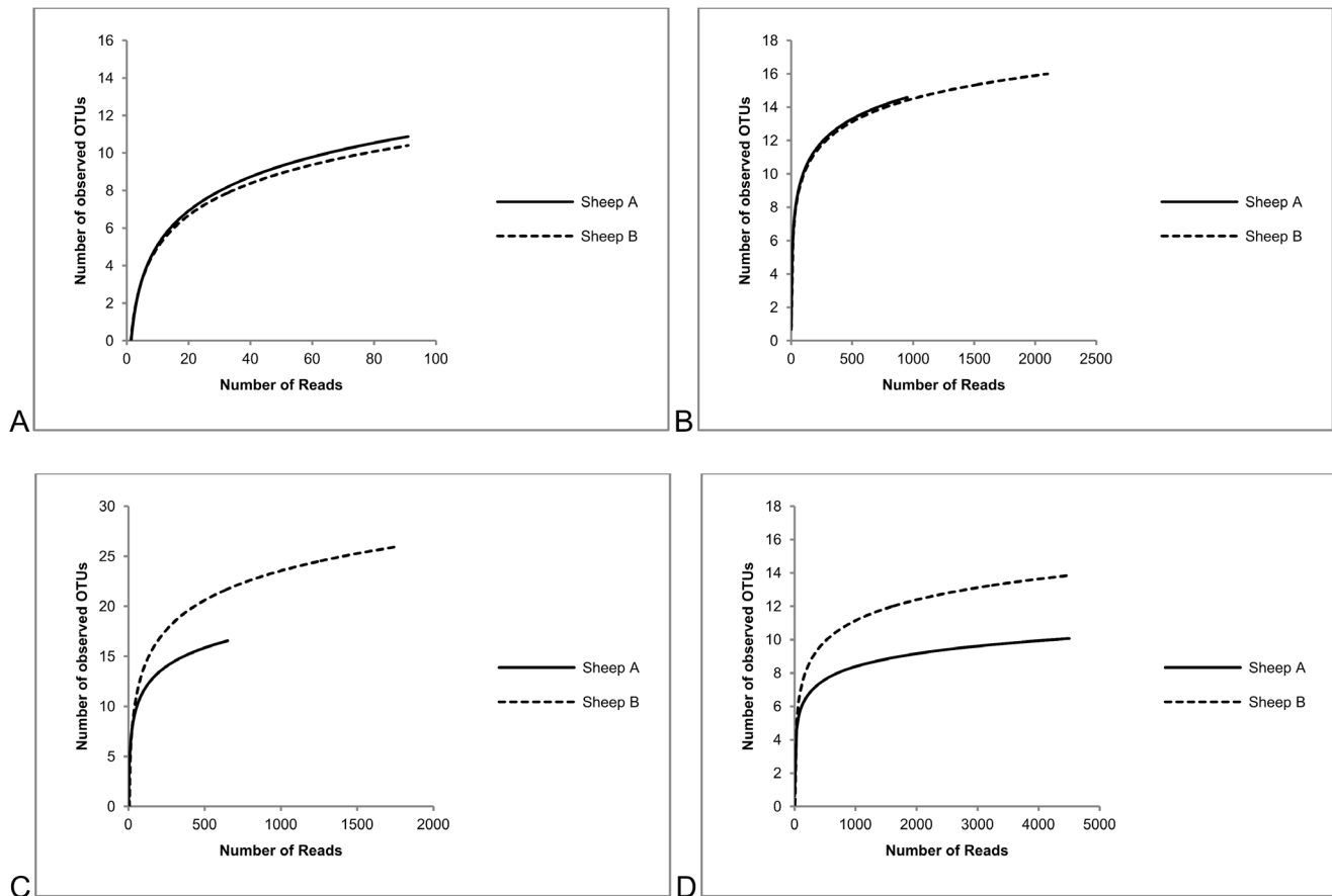
Figure 1. Multiple rarefaction collectors curves. Observed number of OTUs for different sequencing and analysis methods: A. SA rrn . B. IM rrn . C. IM mcrA . D. IA rrn .
