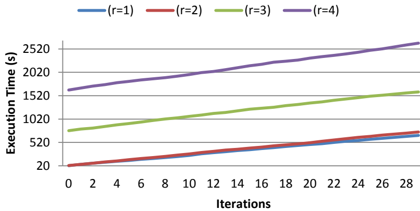
Figure 11 - I-RACOFS timing results for d=3
