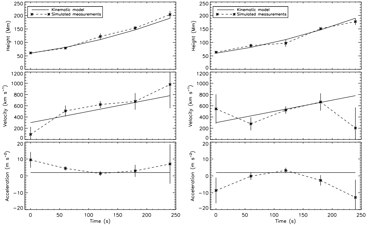
Fig. 1. Kinematic model for a CME with constant acceleration 2 \text{ m s}^{-2} and initial velocity 300 \text{ km s}^{-1} , and two data simulations of how the resulting profiles for different scatters on the height-time measurements ( top panels ) behave when 3-point Lagrangian interpolation is used to derive the velocities ( middle panels ) and accelerations ( bottom panels ). Both simulated cases were produced by adding scatter to the height measurements, via a normally-distributed random number generator with a standard deviation of 10% of the model height at each time-step. The different instances of scatter shown here produce completely opposing trends in the accelerations, with the errorbars failing to appropriately overlap the model, therefore belying the true trend.
