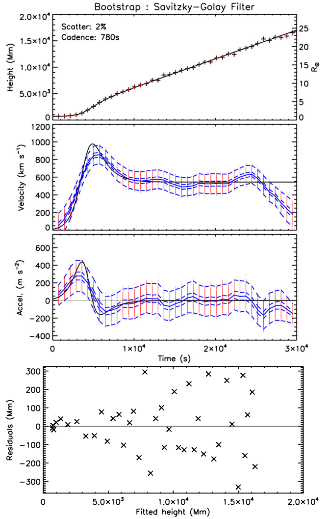
Fig. 8. Bootstrapped Savitzky-Golay filter method applied to the simulated CME height-time measurements as in Fig. 7. This manner of piecewise fit smooths the measurements by fitting a polynomial to the 3 neighbouring points either side of each data point, and is successful in revealing the non-constant acceleration profile. The randomly scattered residuals also indicate its appropriateness.
