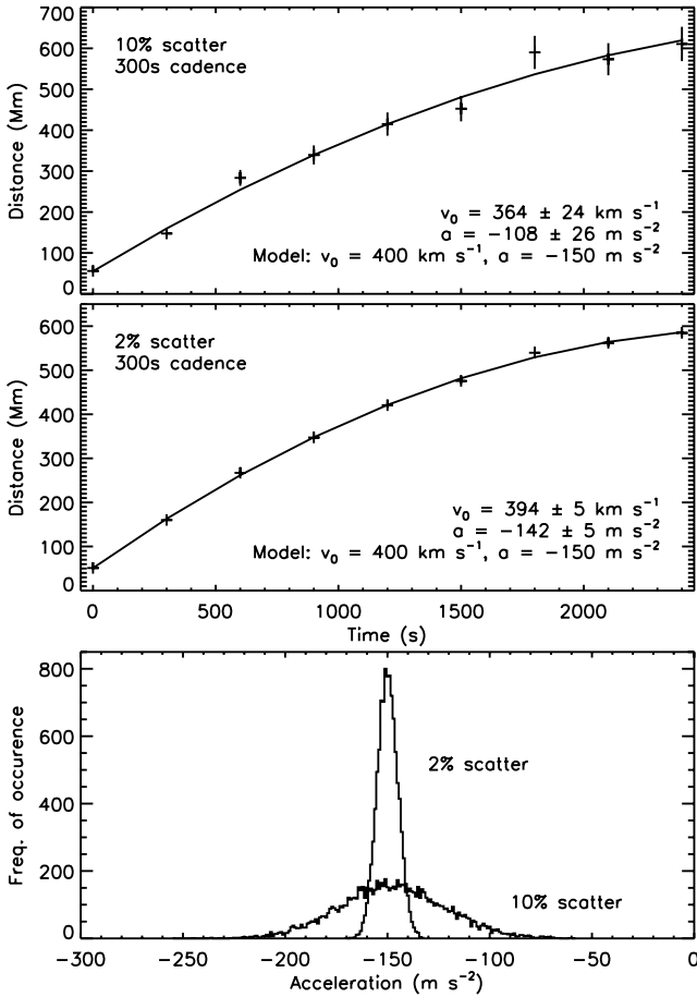
Fig. 2. Simulated distance-time measurements with 3\sigma scatters of \pm 10\% (top), and \pm 2\% (middle) of the model value, at a fixed cadence of 300 s, and the resulting quadratic fit and v_0 and a parameters. The reduced scatter increases the precision for obtaining the true kinematics, as demonstrated by the different distributions of derived acceleration fit parameters from 10 000 runs of the simulation (bottom).
