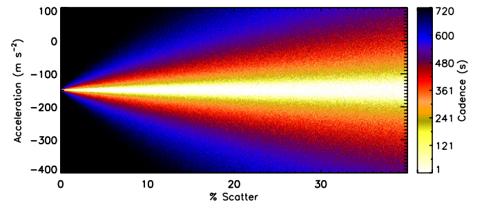
Fig. 4. Simulation of the derived accelerations from the model fits to Eq. (2) (with examples shown in Figs. 2 and 3), for scatters of 0–40% and cadences of 1–720 s. As shown, a decrease in both the data scatter and the cadence time improves the chances of obtaining the correct acceleration value, being -150 \text{ m s}^{-2} in this model coronal wave case.
