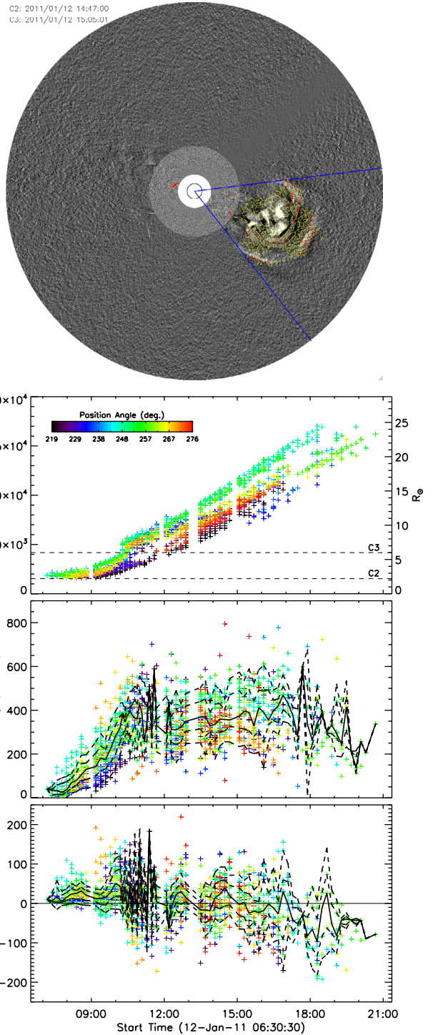
Fig. 10. Savitzky-Golay filter applied to the automated CORIMP CME detection and tracking of an event observed by SOHO/LASCO on 2011 January 12 ( top image ). The detected CME structure is highlighted in yellow, and the outermost height measurements indicated in red. The top plot of the lower panels shows the height-time measurements across the angular range of the CME (indicated by the colourbar). The middle and bottom plots show the derived velocity and acceleration profiles, with the median (solid line), interquartile range (inner dashed lines) and upper and lower fences (outer dashed lines) over-plotted.
