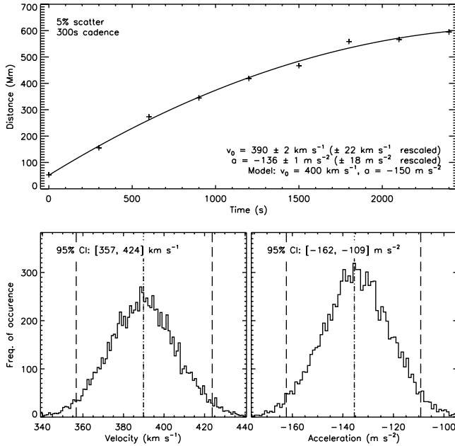
Fig. 6. Top panel: initial fit of Eq. (2) to simulated coronal wave distance-time measurements, with 5% scatter and 300 s cadence. Errorbars of \pm 1.1 Mm are assigned to the measurements, based on the 1.5 arcsec resolution of the imager. The fit parameters are quoted with 1\sigma uncertainties, with the rescaled uncertainties shown in brackets. Bottom panels: histograms of the initial velocity and acceleration values derived using the bootstrapping technique. The mean and 95% confidence interval are indicated by the dot-dashed and dashed lines respectively. Bootstrapping provides a distribution of fitting parameters that is unattainable via a standard single-fit to data when unknown sources of uncertainty exist.
