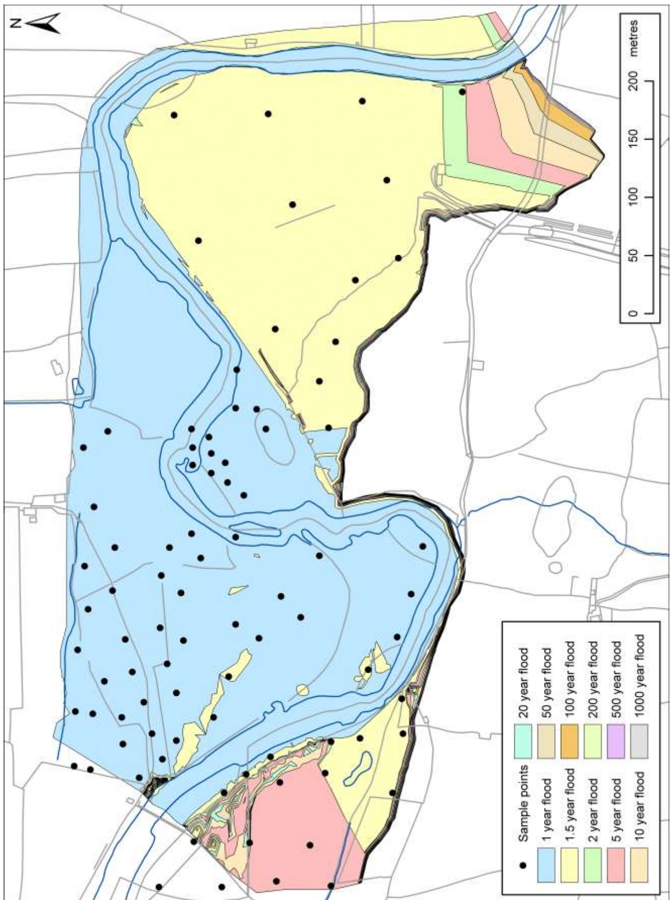
Figure 16: Simulated flood limits at Reeth.
