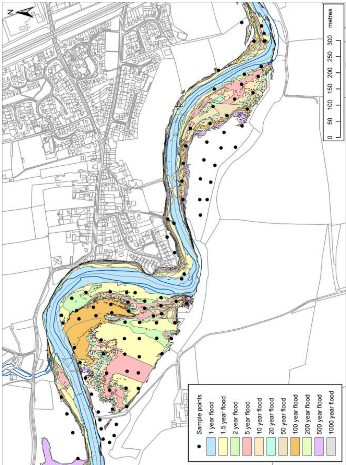
Figure 17: Simulated flood limits at Brompton-on-Swale.
