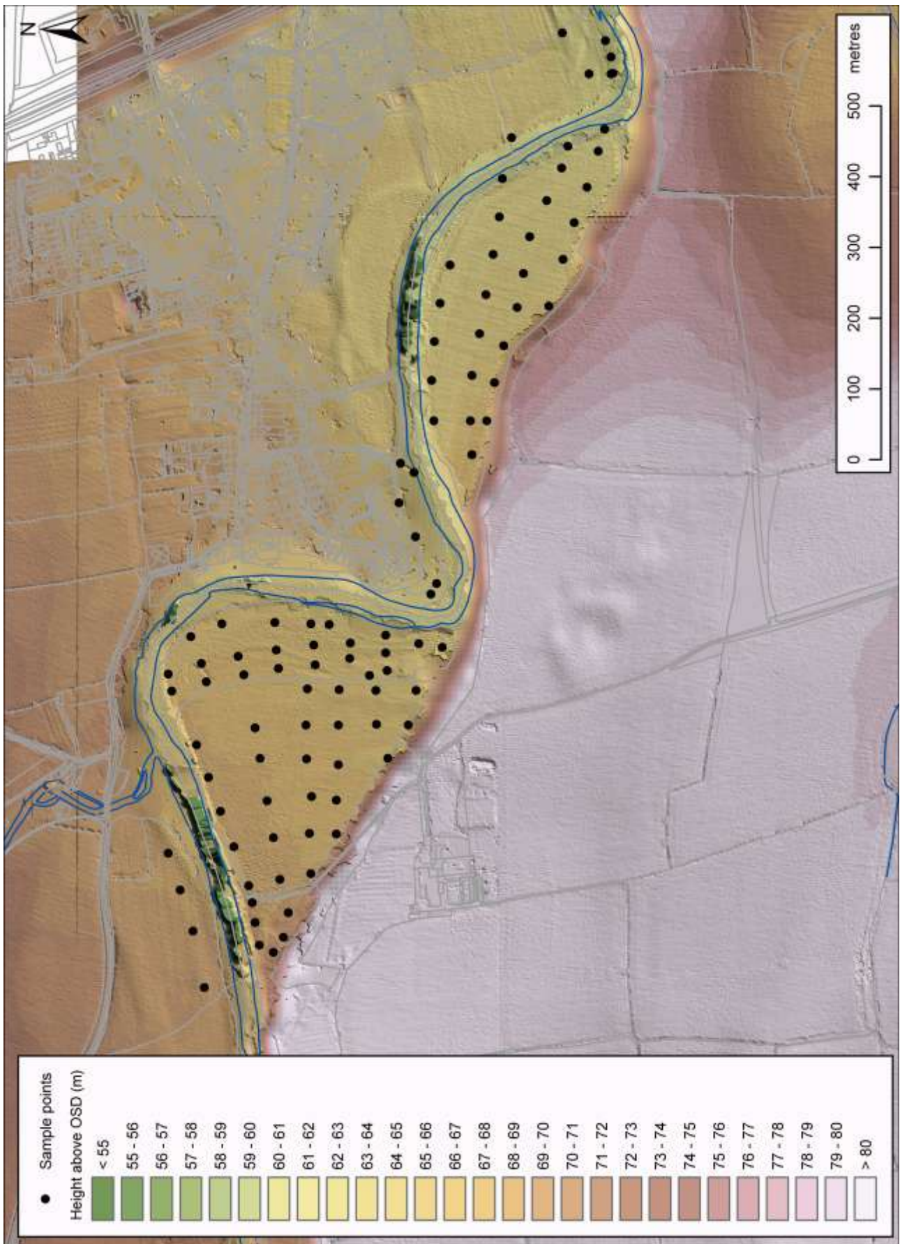
Figure 3: The study reach at Brompton-on-Swale showing geochemical sample point locations.
