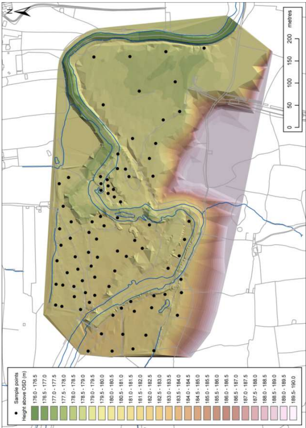
Figure 2: The study reach at Reeth showing geochemical sample point locations.
