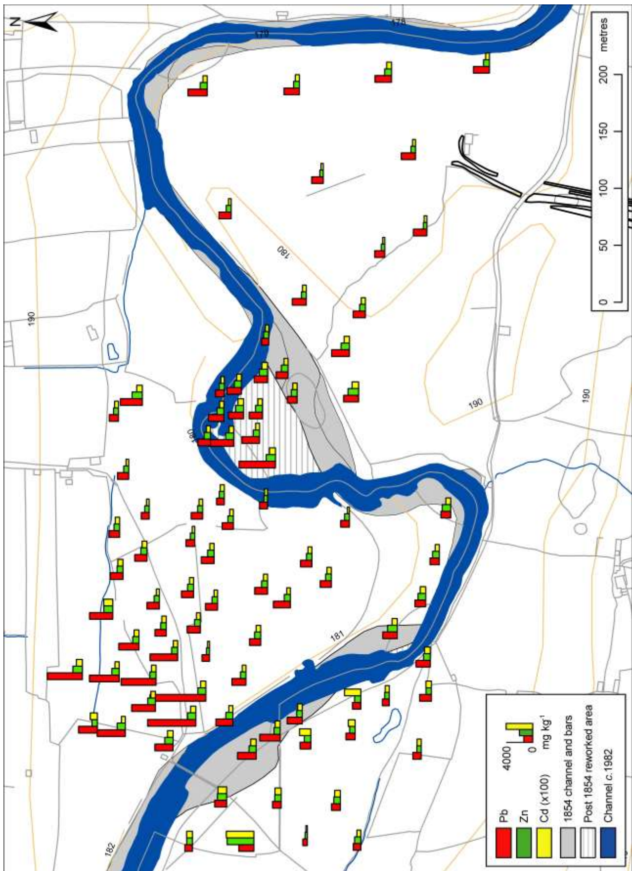
Figure 7(a): Pb, Zn and Cd concentrations in floodplain surface soils at Reeth.
