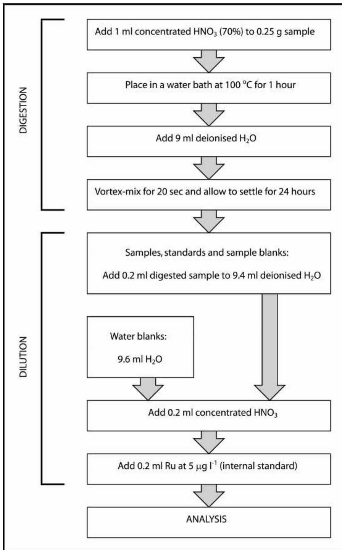
Figure 4: Flowchart illustrating the HNO 3 digestion procedure.
