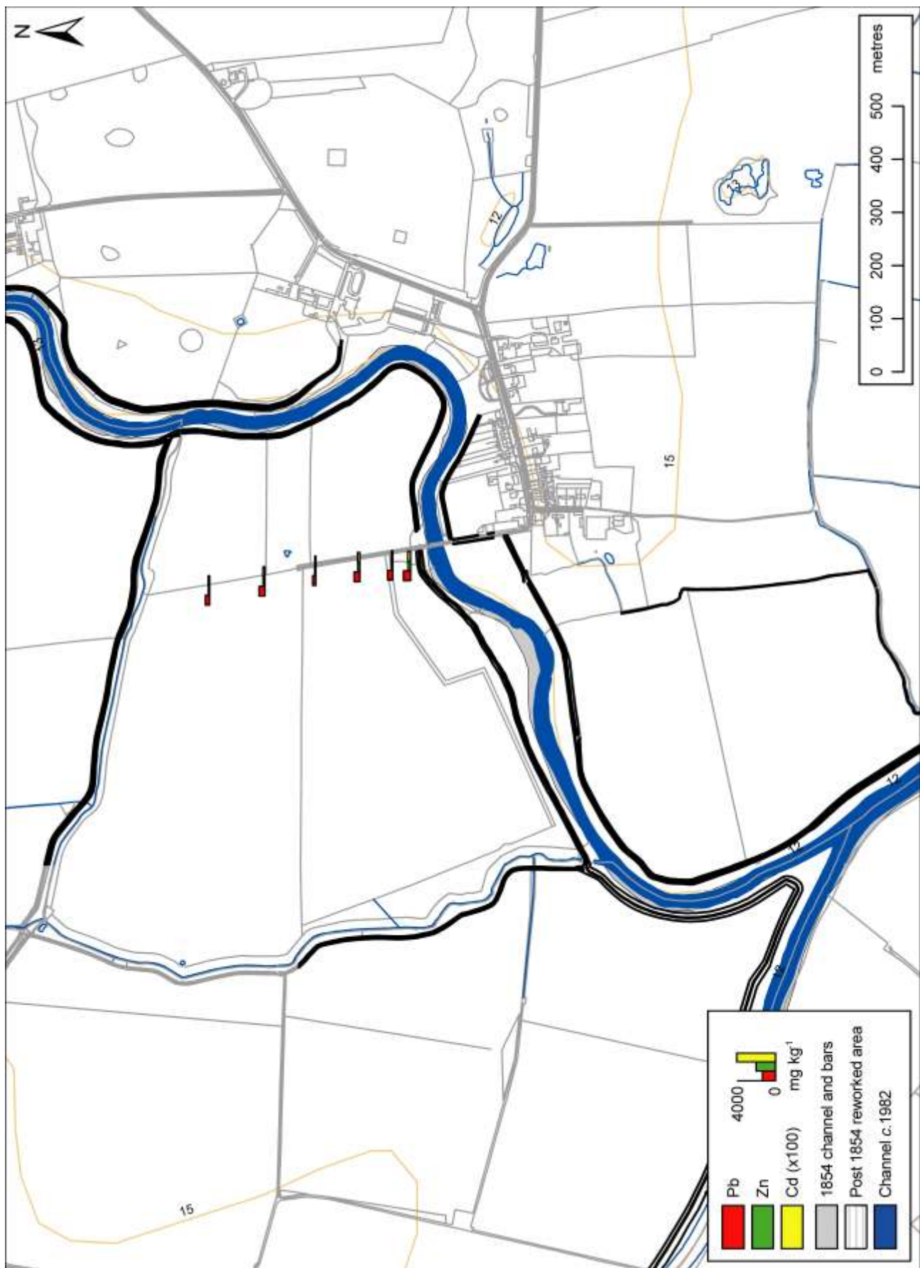
Figure 14(b): Pb, Zn and Cd concentrations in floodplain subsurface soils at Myton-on-Swale.
