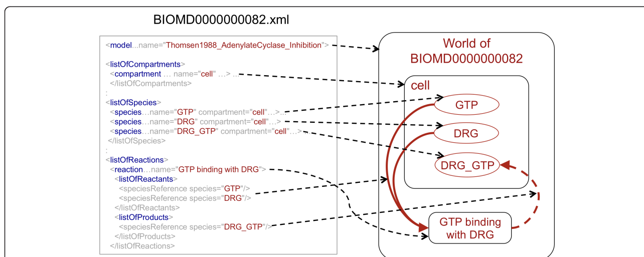
Figure 2 Schematic representation of a part of the representation generated for BIOMD0000000082. Here, we demonstrate part of the transformation of the specification of the model BIOMD0000000082 ( in silico , on the left) into a representation of in vivo phenomena (on the right). Each line represents an explicit assertion we create and by which knowledge that is currently implicit in the SBML code is made explicit in an ontology-based, formal representation. The World of BIOMD0000000082 has, as a part, a Cell (represented by the model's component). The Cell has, as its parts, three species (represented by "GTP", "DRG" and "DRG_GTP"). The reaction "GTP binding with DRG" represents a process that occurs in the World of BIOMD0000000082 and has as input the objects represented by "GTP" and "DRG", and has as output the object represented by "DRG_GTP". The input and output relations for processes are inferred from the SBML list of reactants and products, respectively.
