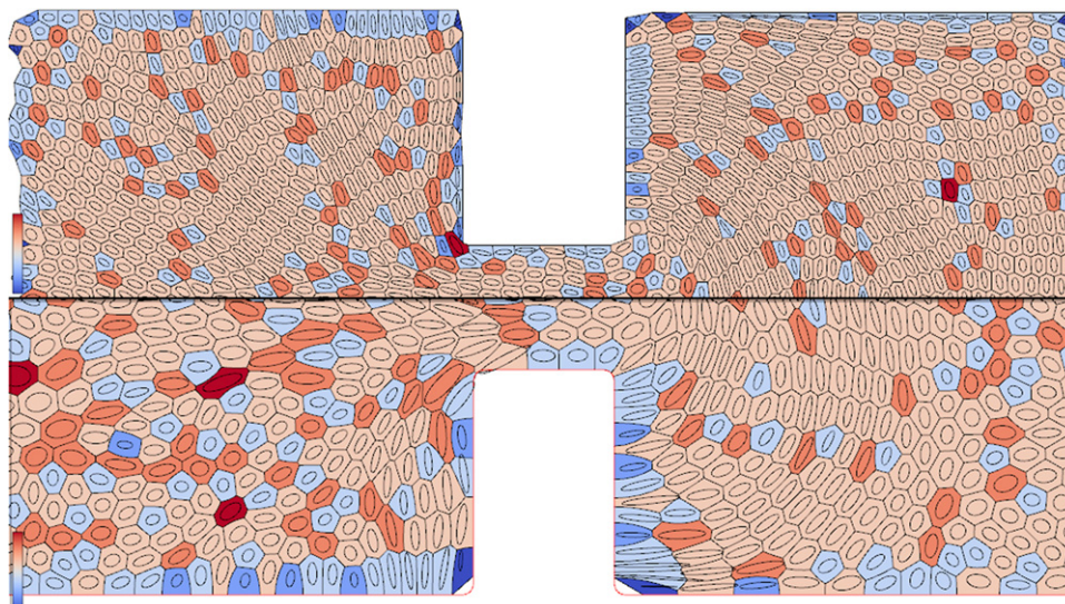
Fig. 7. A photograph of an experiment in which a foam flows through a constriction can be reconstructed in Surface Evolver [12], and then visualized in FoamVis. Here we compare such an experiment (top) with a simulation (bottom), as described in Section 3.2. Each bubble is coloured by its number of sides, and contains an ellipse indicating the direction and magnitude of the local strain. Note that there are many more bubbles in the experiment, and that the strain is lower, presumably because of the finite liquid fraction.
