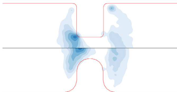
Fig. 3. Flow of a foam through a 4:1:4 constriction, showing a smoothed profile of T1 density. The cumulative distribution of T1s changes when the corners of the constriction are either sharp (top) or rounded (bottom). It is apparent that there are more T1s upstream than downstream, and that for the case of a sharp corner most T1s occur close to the corners and the maximum in T1 intensity is shifted upstream.
