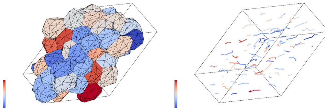
Fig. 6. Quasistatic simple shear of a polydisperse dry three-dimensional foam of 65 bubbles, with periodic boundary conditions (shown as a parallelepiped, cf. [17]). Using the multiple views feature, FoamVis animates the foam on the left and shows the corresponding bubble paths on the right. Bubbles and paths are coloured by bubble volume. Sudden changes in path direction are a result of T1s.
