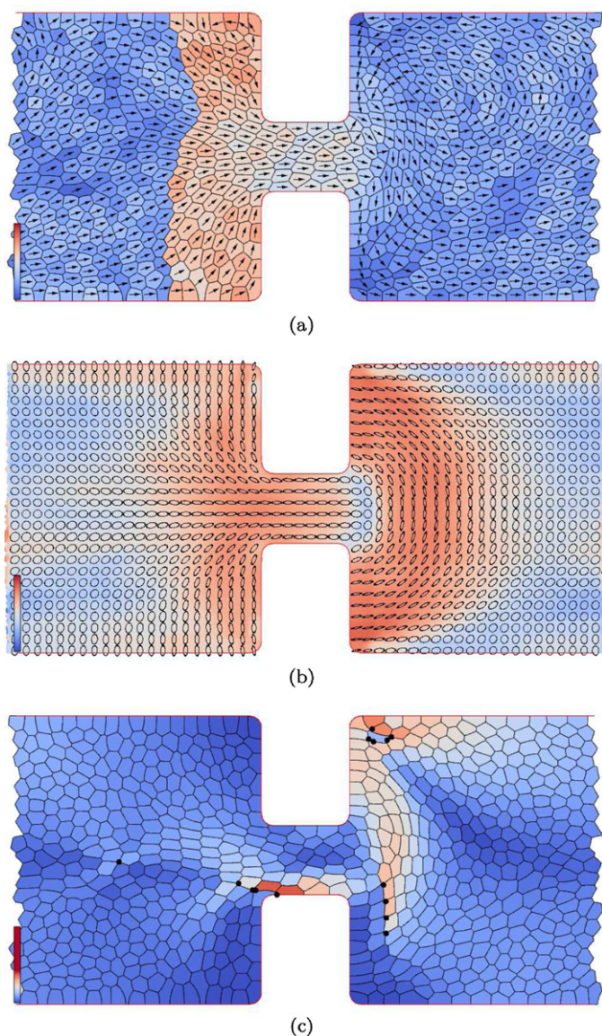
Fig. 2. Flow of a foam through a 4:1:4 constriction from left to right. (a) Bubbles coloured by instantaneous pressure, with their direction of motion (velocity vectors with equal length) indicated. Note the region of high pressure just upstream of the constriction, and the apparent vortex in one of the upstream corners. (b) A rolling average of the texture tensor (ellipses), with pixels coloured by the average of its largest eigenvalue, indicating the local strain. The foam is isotropic far from the constriction, but the bubbles are elongated parallel and perpendicular to the direction of flow up- and downstream respectively. (c) Bubbles with large instantaneous velocities appear to correlate with the position of T1s (black dots); it is also apparent that T1s often occur in avalanches, and that their effect on bubble motion is extensive.
