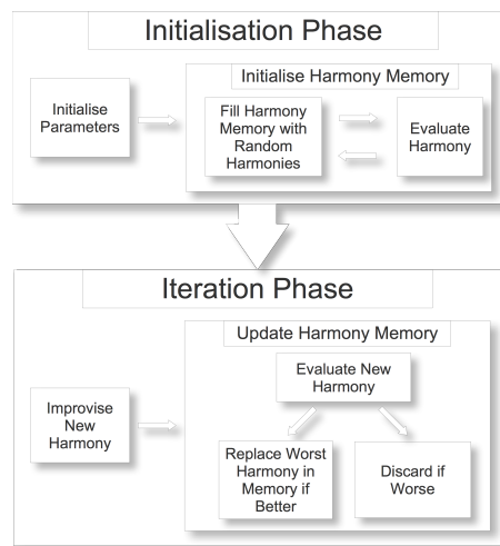
Fig. 2. Illustration of Harmony Search
