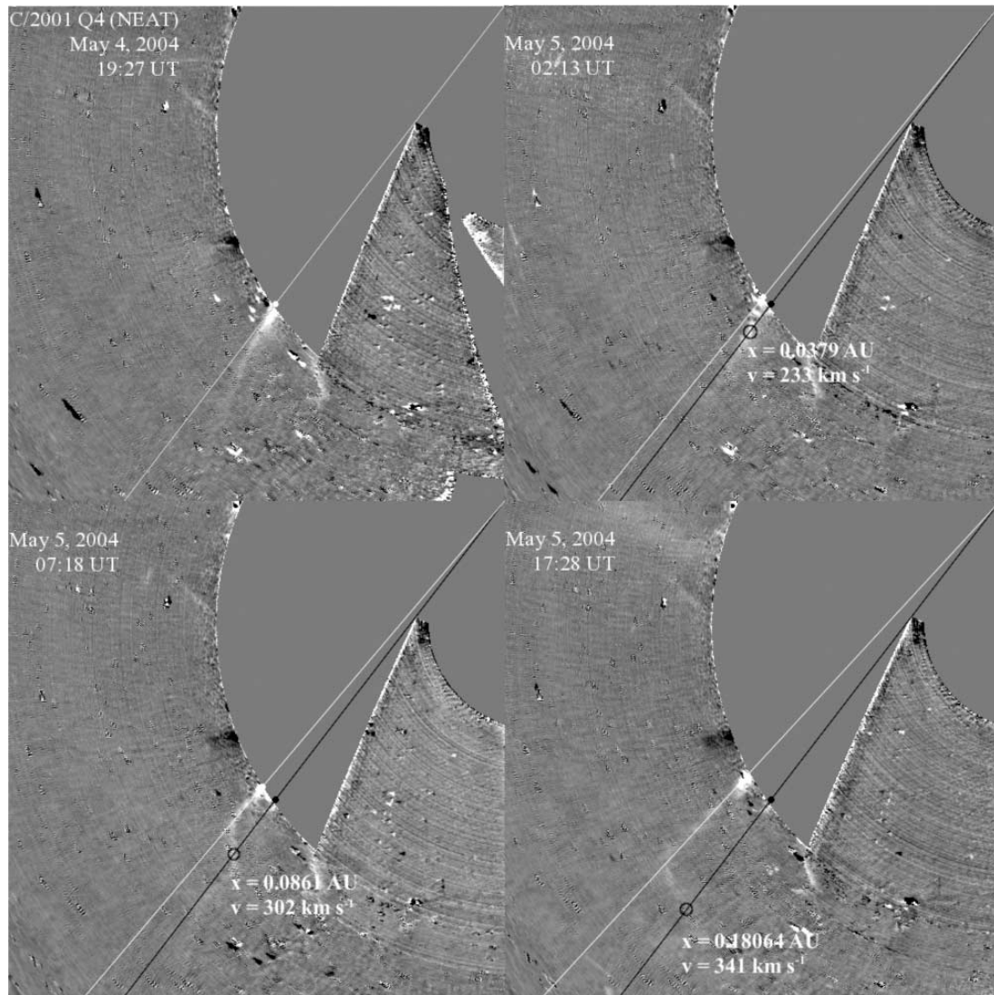
FIG. 5.—Four sections extracted from separate Sun-centered fisheye sky maps. The Sun is located in the top right corner of each frame, and a white line is plotted from the Sun to the comet's nucleus for each frame. This line plotted along the Sun-comet line for the first frame is kept fixed as a black line in subsequent frames, and is used as the reference point for radial velocity measurements; a new white line is plotted along the Sun-comet line of the current (new) frame. Intersection of the comet tail with the black line is indicated by a circle. The radial velocity values here are determined by the angle between this circle and the black dot marking the comet's position in the initial frame, converted to a distance (as in Fig. 2) and divided by the time between the two maps.
