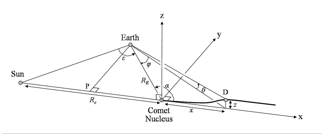
FIG. 2.—Comet coordinate frame; the nucleus is at the origin. The x -axis connects the Sun and the nucleus as shown, with positive pointing away from the Sun. Point “P” is the location where the x -axis is closest to Earth. The x - z plane is perpendicular to the line connecting P and Earth. In this coordinate frame the comet tail remains close to the positive x -axis. Locations in the sky near the comet, such as point “D”, as seen from Earth, are specified by the two angles (\phi, \theta) , where \phi is the spherical coordinate “longitude” of the given point along the comet’s tail, positive away from the Sun, and \theta its “latitude.” For the observations presented here, point P is usually (but not always) located as shown between the Sun and comet nucleus on the negative x -axis. Note that this coordinate frame follows the motion of the comet nucleus relative to the Sun and Earth.
