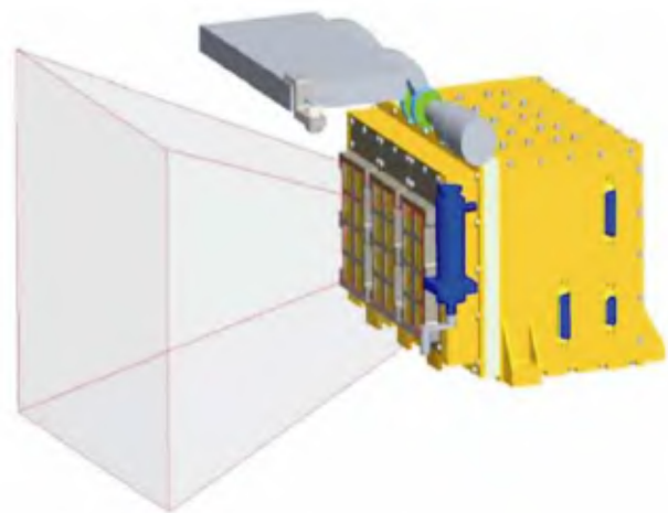
Figure 1. Design image of the C1XS instrument showing colligned front detectors, deployable radiation shield and 14^{\circ} field of view. Note white thermal gasket separating cool detector enclosure from electronics.
