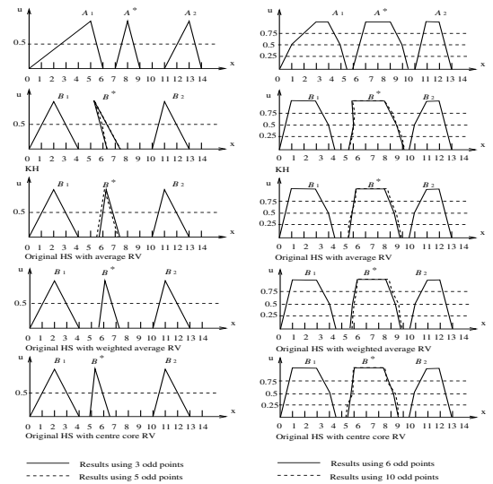
Fig. 6. Examples of piecewise linearity for KH and original HS method
