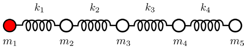
Figure 1. Indirect classical system tomography of a quadratic Hamiltonian. In this example, the spring constants k_i and masses m_i of a chain of coupled harmonic oscillators can be determined by monitoring the dynamics of a single particle at the chain end (in red). See [1] for details.
