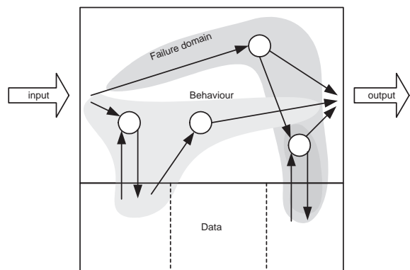
Figure 1: Failure domain localisation in software
