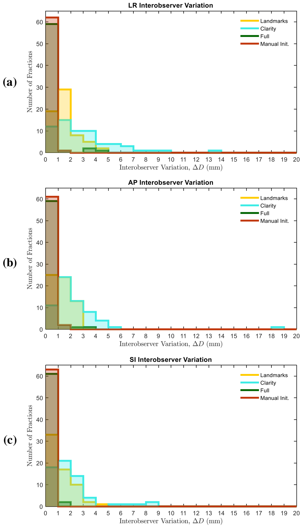
Figure 3. Histograms of interobserver variation ( \Delta D ) in match results for Clarity, Full and Manually Initiated workflows, with Manual Landmark matches for reference.
