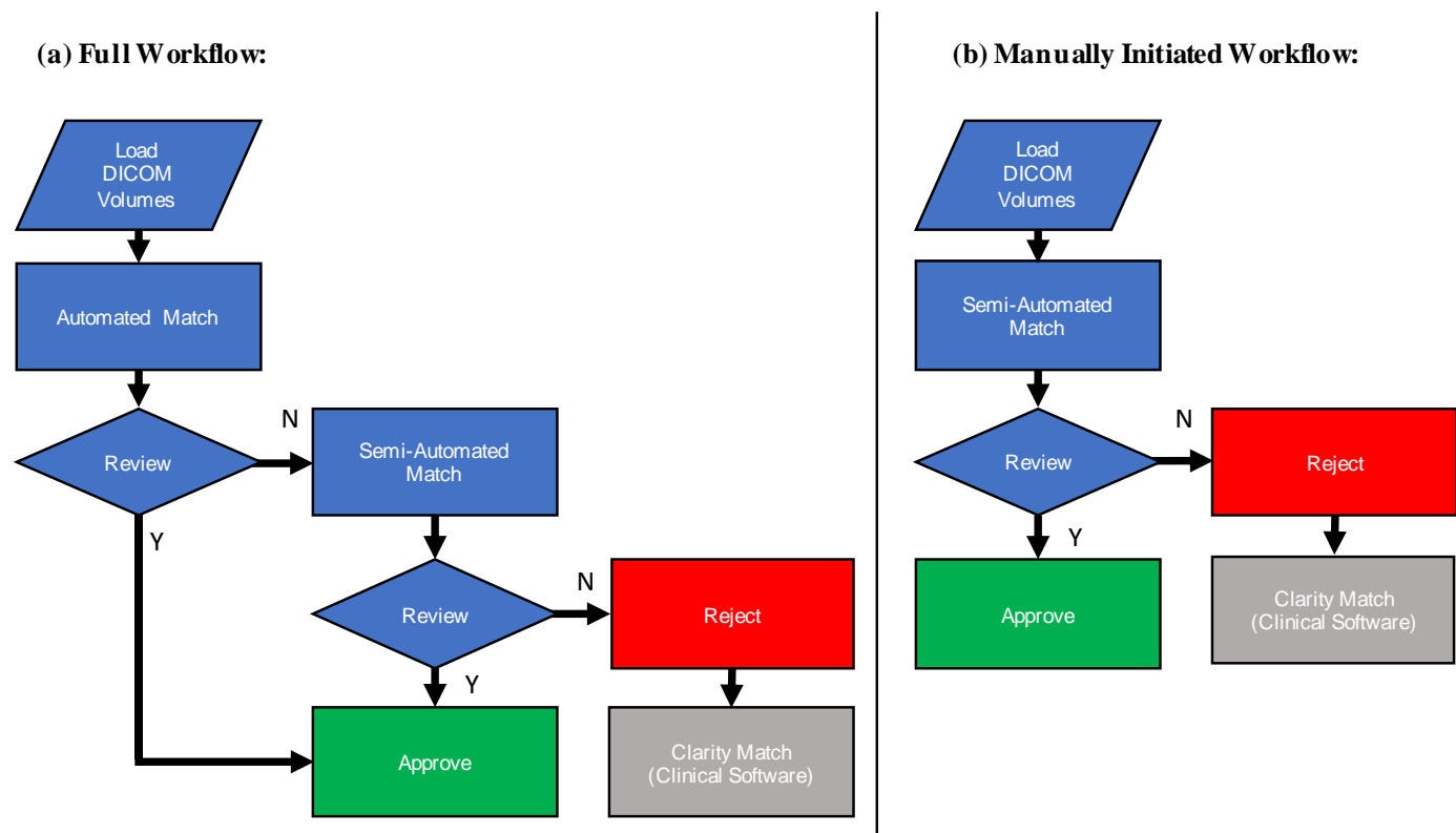
Figure 1. Flowcharts for the two semi-automated matching workflows: (a) Full workflow and (b) Manually Initiated workflow.
