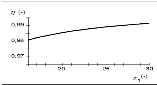
Fig. 7. Dependence of gearing efficiency on pinion teeth number at constant value of transverse gearing load
