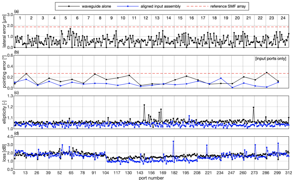
Fig. 4 (a) Lateral positioning errors of the waveguide core positions; (b) pointing errors of the input channel beams to the waveguide facet normal; (c) ellipticity of the free-space beams; (d) insertion losses from the input fibres to the free space beams.
