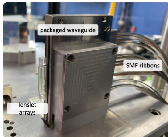
Fig. 5 A detailed view of the input/output optics assembly.
