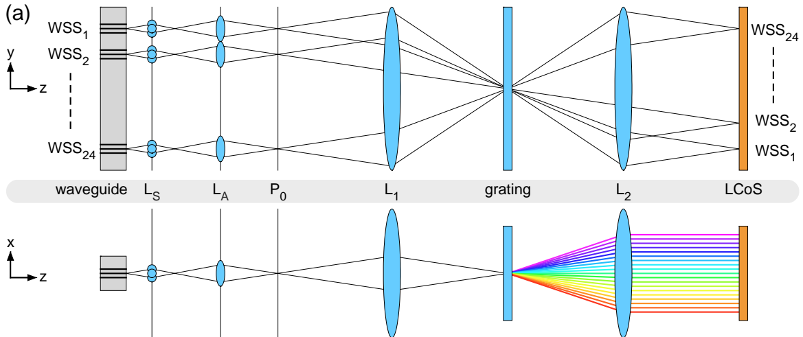
Fig. 1 The optical architecture of stacked WSS module.
