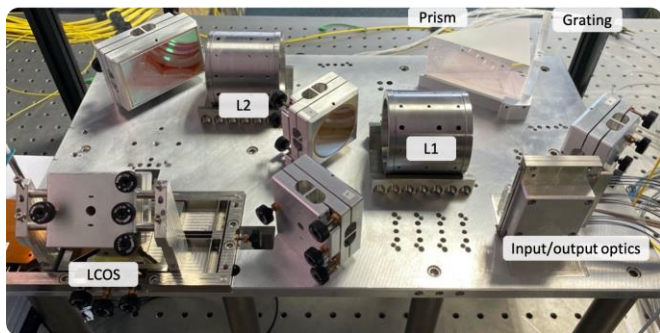
Fig. 3 The experimental setup of the 24 1 \times 12 WSS module
