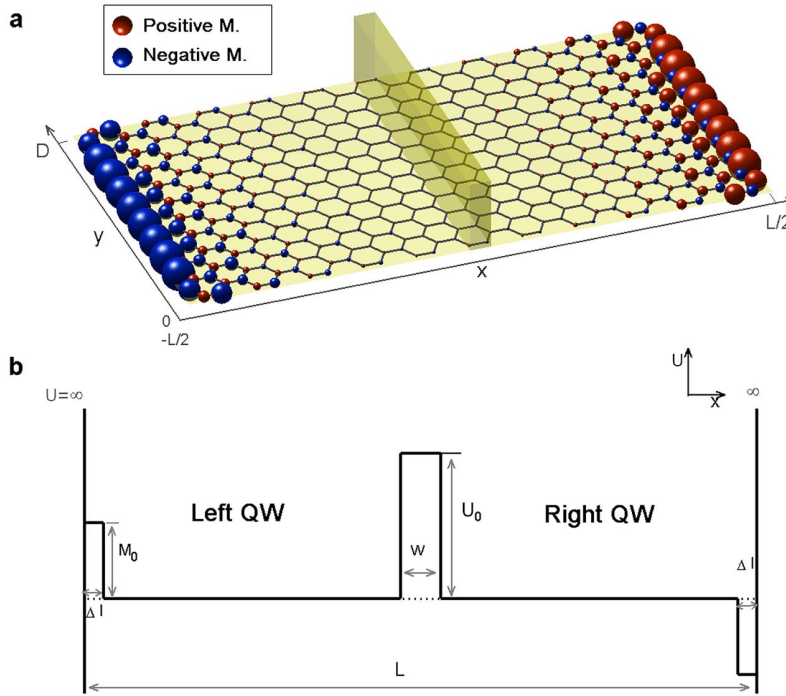
FIG. 64. System setup for mean-field analysis of the emergence of polarized states. (a) Illustration of a rectangular graphene domain of length L and width D with a potential barrier in the middle. The zigzag and armchair edges are along the y - and x -axis, respectively. The filled red (blue) circles at the right (left) zigzag boundaries denote the positive (negative) magnetic moments, the radii of which represent the strength of spin density. (b) The effective potential profile \tilde{U}_\uparrow(x) at the position y = D/2 for spin-up electrons, where the positive and negative potentials near the boundaries represent the strength of the respective spin density, which approaches the value of M_0 ( -M_0 ) at the left (right) zigzag edges in (a). The effective potential for spin-down electrons is reversed at the boundaries as compared with that for spin-up electrons. From Ref. [136] with permission.
