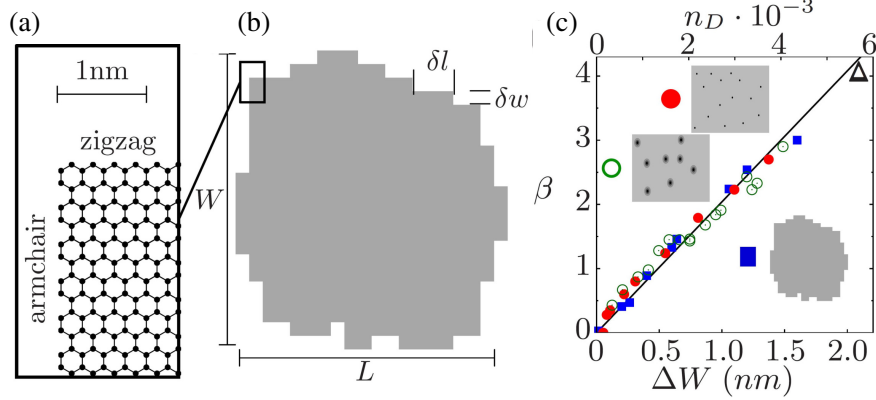
FIG. 13. Level spacing statistics of a graphene flake in the absence or presence of random disorders. (a) A rectangular segment of a graphene flake with armchair vertical and zigzag horizontal edges. (b) Approximately rectangular quantum dot with rough edges. (c) Dependence of parameter \beta characterizing the transition from a Poisson to a GOE distribution on the edge roughness amplitude \Delta W (squares), and the density of short-range ( n_D , full circles) or of long-range ( n_C = 4n_D , rescaled for visual clarity only, open circles) impurities. From Ref. [286] with permission.
