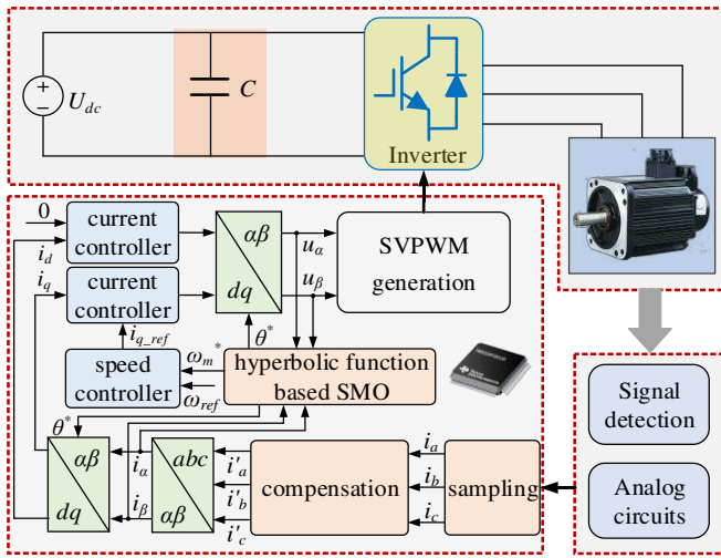
\omega_{ref} : reference speed U_{dc} : DC voltage i_{d\_ref}, i_{q\_ref} : reference currents
