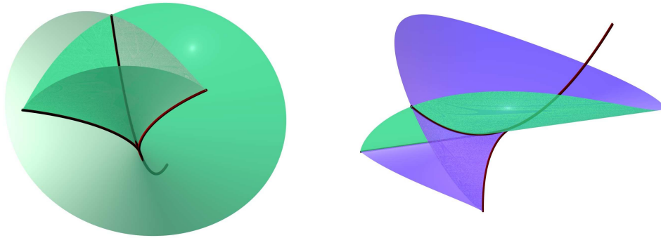
FIGURE 3. The swallowtail.
