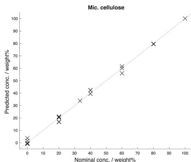
Fig. 7. The predicted leave-one-out cross validation results for the raw EDXRD data of unpackaged tablets for the three compounds.
