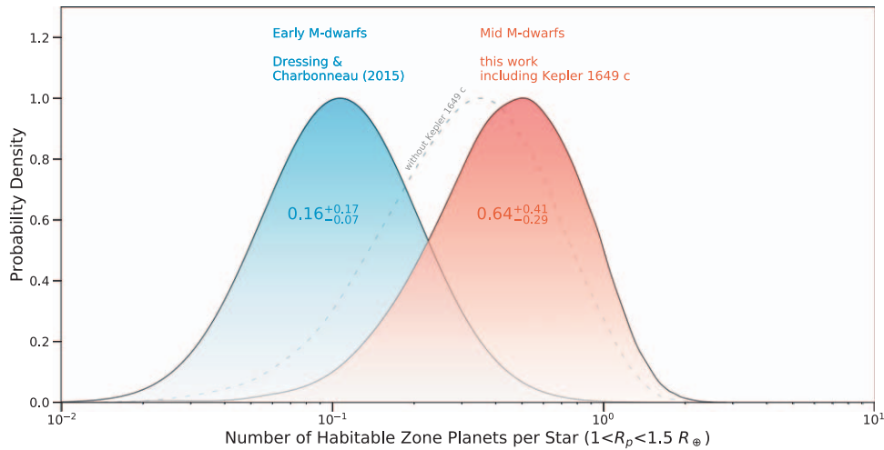
Figure 3. Posterior probability distributions on the occurrence rate of planets between 1 and 1.5 R_{\oplus} in size in their stars’ conservative habitable zones. We show both the occurrence rate for these planets around early M-dwarf stars (blue distribution) from Dressing & Charbonneau (2015), and mid M-dwarf stars (red distribution), including Kepler-1649 c in the calculation. We approximated the posterior distribution for early M-dwarf stars by finding (via least squares minimization) a log-normal distribution whose median and 68% confidence intervals most closely matched (within about 1%) those reported by Dressing & Charbonneau (2015). We also show the posterior probability distribution for mid M-dwarfs without including Kepler-1649 c as a gray dashed line. The addition of Kepler-1649 c slightly increases the measured occurrence rate of small, habitable-zone planets around mid M-dwarfs and adds new evidence suggesting that these planets may be more common than those around higher-mass stars.
