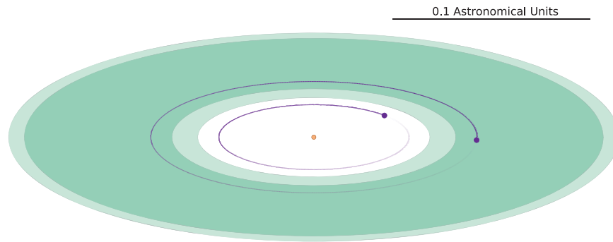
Figure 2. Diagram of the Kepler-1649 system, from the vantage of an observer inclined by 20 degrees from the plane of the system. The host star, Kepler-1649, is shown to scale in the center of the image, colored as a 3200 K blackbody would appear to the naked eye (see http://www.vendian.org/mncharity/dir3/blackbody/UnstableURLs/bbr_color.html ). The optimistic and conservative habitable zone defined by Kopparapu et al. (2013) are colored in light and dark green, respectively. The orbits of Kepler-1649 b and c are shown as faded purple curves. The purple dots at the ends of the orbit curves denoting Kepler-1649 b and c are not to scale; the planets’ true sizes would be about 4 times smaller than the orbit curve widths.
