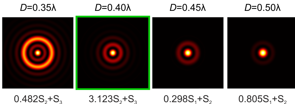
FIG. 4. Engineering of superscillatory hotspots. A range of superscillatory spots showing the flexibility of the design algorithm with a varying spot size. The superscillatory spot used in the biological imaging is highlighted in green. Below each spot is the equation describing the construction of the spot from circular prolate spheroidal wavefunctions.
