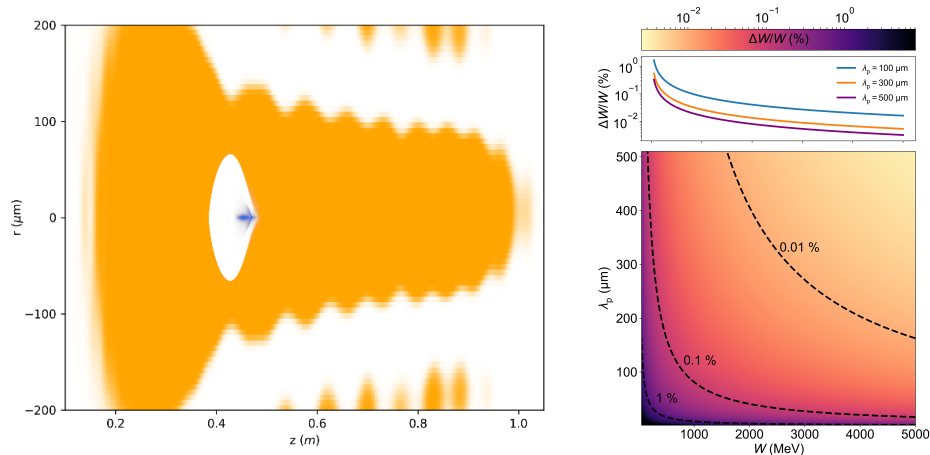
Figure 3. Left panel: A much wider plasma channel (orange) than in E-210, thus being able to accommodate a much longer plasma wavelength PWA-structure (white), driven by a FACET-II sized electron beam (blue) propagating to the right. Right panel: Longer plasma wavelengths \lambda_p allow the plasma photocathode to generate electron beams with smaller absolute energy spreads, based on a scaling law from Ref. 10, which allows reaching sub-0.01% relative energy spreads already at few GeV electron energies, which are today routinely reached by modern plasma accelerators in single stages.
