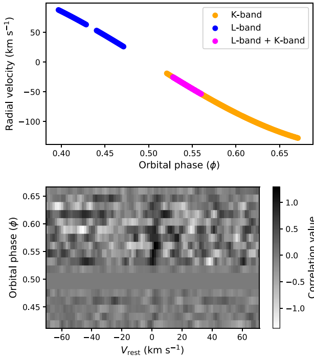
Figure 7. Top: Radial velocity of HD 179949 b as a function of the observed orbital phases in the L -band (blue circles) and K -band (orange circles), and the phases observed with both data sets (magenta circles). This planet radial velocity does not include the velocity corrections for an observer on earth. Bottom: Phase binned cross-correlation values of the combined data set with both bands with their respective best-fitting model atmospheres, shifted to the planet rest-frame velocity. The gap in the right-hand panel corresponds to the large gap in the phase coverage shown in the top panel. There is a noticeable trail of positive correlation values at V_{\text{rest}} \approx 0 \text{ km s}^{-1} indicating a detection of the atmosphere of HD 179949 b.
