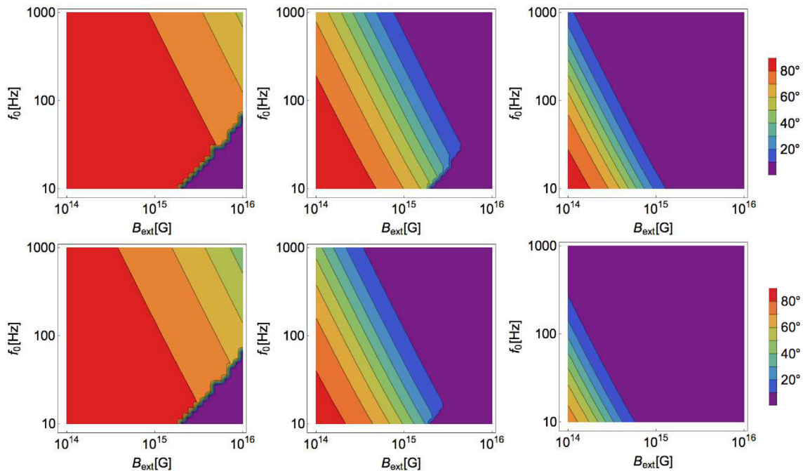
Figure 6. Distribution of \chi (colour scale) for magnetars with an alignment torque prefactor of (from left to right) k = 1, 2, and 3 ; and at ages of 1000 (top panels) and 5000 yr (bottom panels). As before, \chi_0 = 1^\circ and B_{\text{int}} = B_{\text{ext}} for all models.
