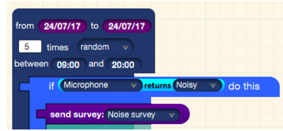
Fig. 3. A combination trigger, based on time and sensor data
