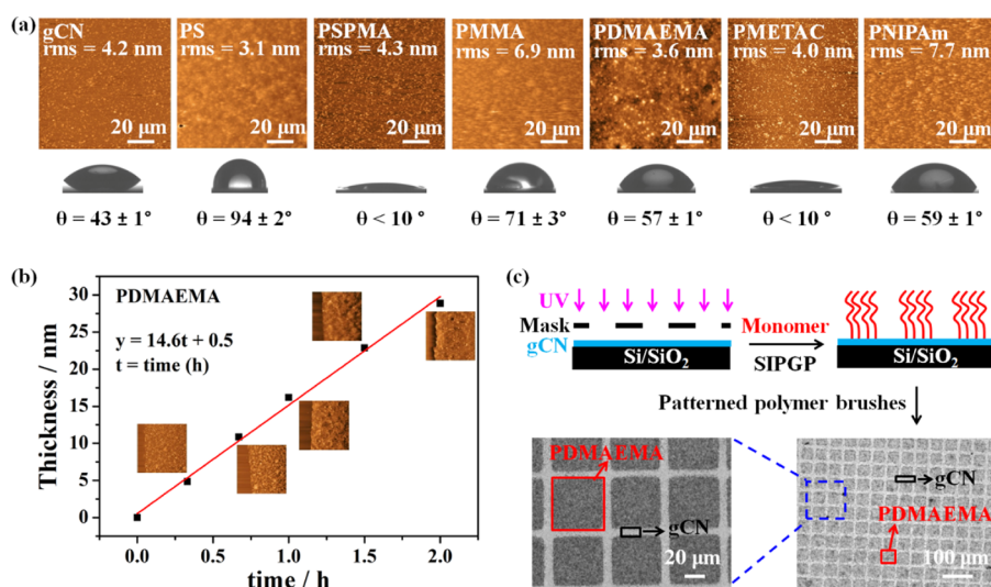
Figure 3. (a) AFM images and water contact angle of gCN and polymer-modified gCN. (b) Thickness evolution of polymer brushes grafted on gCN as a function of polymerization time for PDMAEMA brushes (PDMAEMA as a model system). (c) Schematic illustration and optical photographs of patterned PDMAEMA brushes on a spin-coated gCN film.
