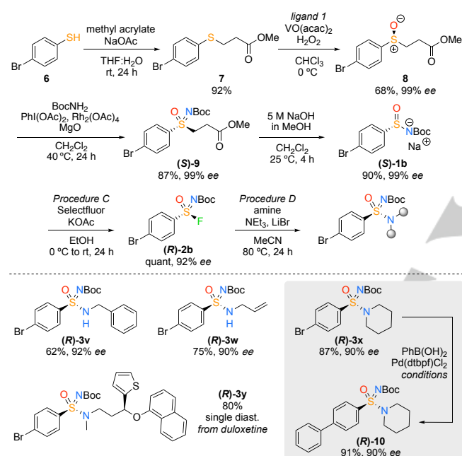
Scheme 4. Preparation enantioenriched 4-bromophenyl sulfoximides. Ligand 1 = ( S )-(-)-2-( N -3,5-diiodosalicyliden)amino-3,3-dimethyl-1-butanol. Stereochemistry of 8 assigned based on prior literature. [30] Suzuki conditions = PhB(OH) 2 (1.5 equiv), K 2 CO 3 (2 equiv), Pd(dtbpf)Cl 2 (10 mol%), MeCN:H 2 O (1:1, 0.2 M), 80 °C, 2 h.
