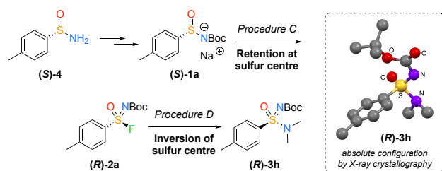
Scheme 3. From the commercially available ( S )-enantiomer of the sulfinamide salt building block, the fluorination-amine coupling sequence was proven to occur with overall inversion of the sulfur centre from crystal structure analysis, rationalized to occur in the amine coupling step.
