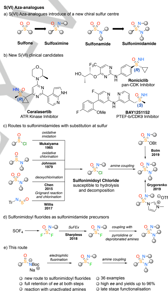
Figure 1. Structure of sulfoximine and sulfonylimidamide groups and S(VI) clinical candidates with asymmetric sulfur centres. Synthetic routes to access sulfonylimidamides typically rely on sulfonylimidoyl chloride precursors, alternative sulfonylimidoyl-X species, and this work as a new way to access enantioenriched sulfonylimidoyl fluorides and sulfonylimidamides.
