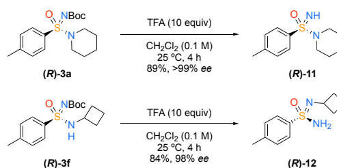
Scheme 6. NBoc-deprotection of primary and secondary sulfoximidoamine. Sample of ( R )- 3f used had 98% ee, with NBoc-deprotection occurring with complete preservation of ee.
