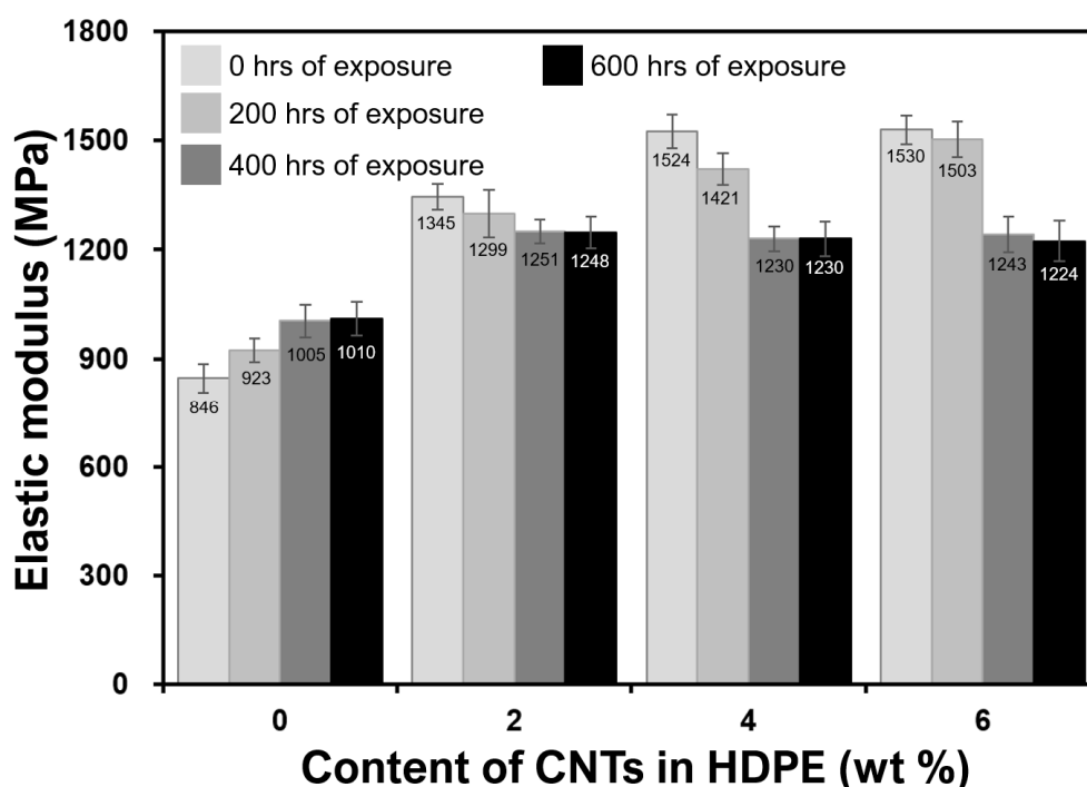
Figure 3. Effect of weathering on elastic moduli of monolithic and nanocomposite samples.
