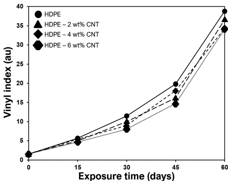
Figure 7. Vinyl indices ( I_v ) of the monolithic and nanocomposite films exposed to UV-B radiation.
