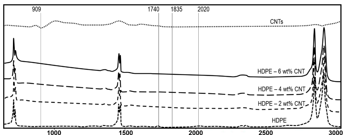
Figure 5. IR spectrum of HDPE, CNTs and nanocomposite films without exposure to UV radiation.
