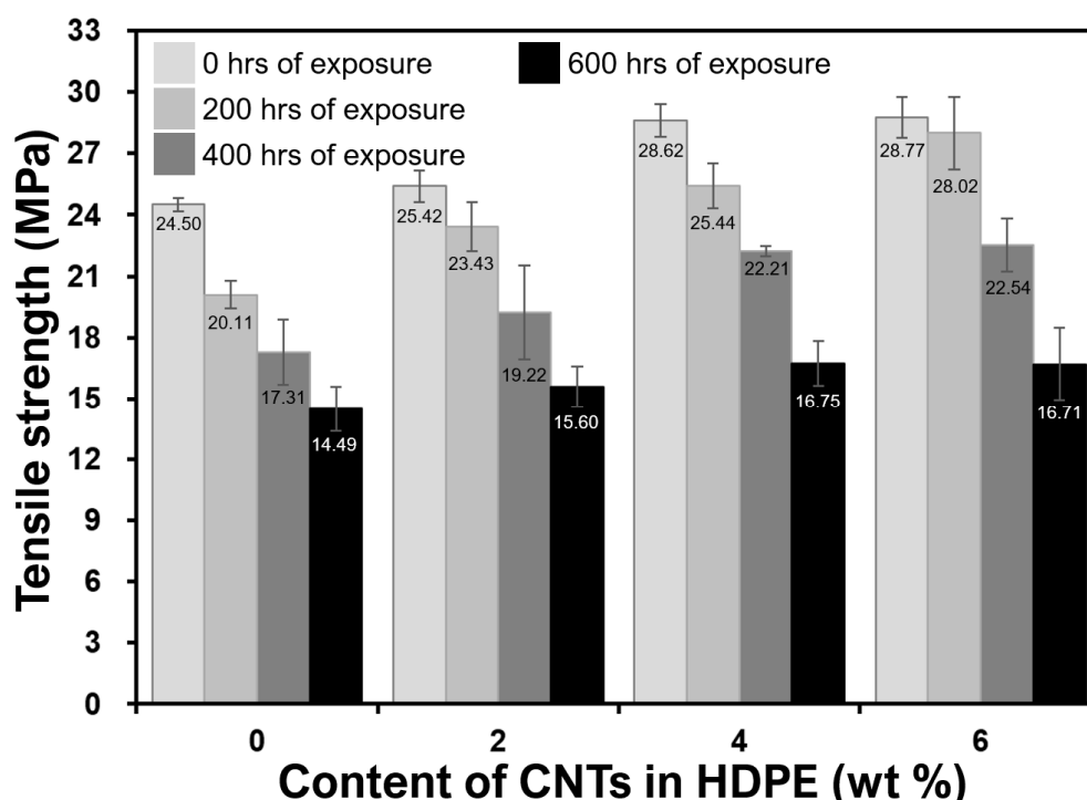
Figure 4. Effect of weathering on tensile strengths of monolithic and nanocomposite samples.
