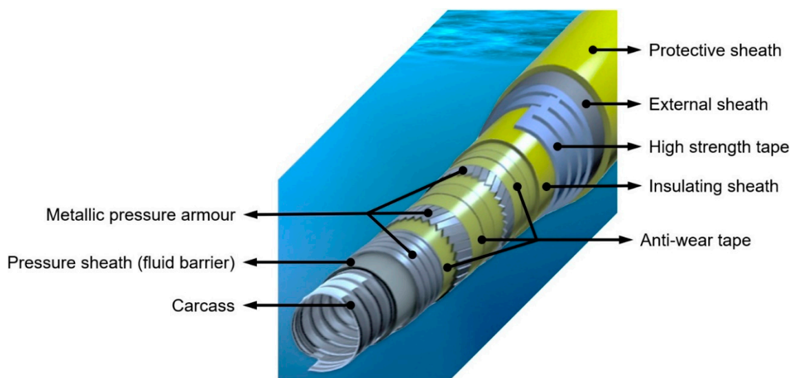
Figure 1. Schematic of a typical flexible umbilical cable for offshore engineering.
