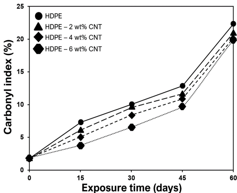
Figure 6. Carbonyl indices ( I_{co} ) of the monolithic and nanocomposite films exposed to UV-B radiation.
