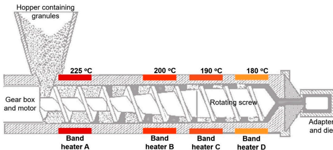
Figure 8. Schematic of extruder with heating temperatures used in this work.
