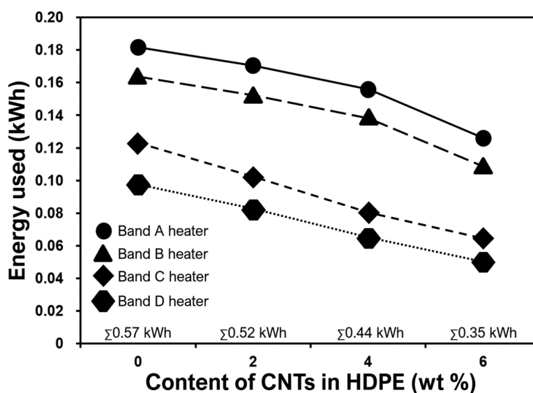
Figure 9. Energy used by respective band heaters for a complete 10 min extrusion cycle. The total energy, the sum ( \Sigma ) of energy data points for every concentration, is on the horizontal axis line.
