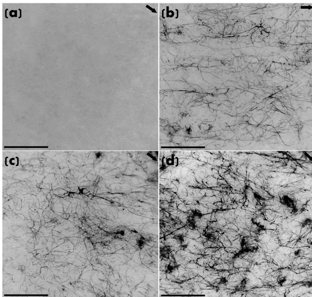
Figure 2. Representative TEM images for: (a) monolithic HDPE; and nanocomposites containing: (b) 2 wt% CNTs; (c) 4 wt% CNTs; and (d) 6 wt% CNTs. Direction of extrusion is represented by the arrow on the top right. Scale bar represents 500 nm.
