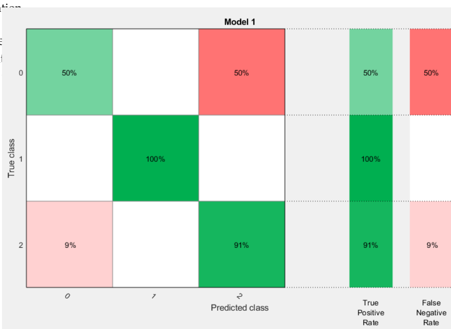
Figure 13. Accuracy of linear discriminant using the confusion for the second dataset with no validation.
