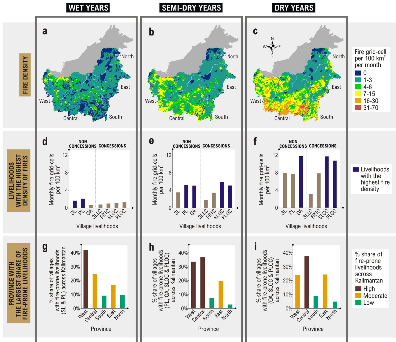
Fig. 5. Fire distributions in relation to climate and village livelihood sectors. (a-c) Density of 1×1 km 2 grid-cells with fires per village per month, (d-f) livelihood sectors with the highest density of fires, and (g-i) province with the largest share of fire-prone livelihoods, by precipitation condition over May-October in any given year: wet (precipitation >250 mm/month, occurred in 2007, 2008, 2010, 2016, and 2017), semi-dry (precipitation 200-250 mm/month, occurred in 2003, 2005, 2011, 2012, 2013, and 2014), and dry years (precipitation <200 mm/month, occurred in 2002, 2004, 2006, 2009, and 2015). Cut-off thresholds for defining high (>25%), moderate (10-25%), and low (<10%) share of fire prone livelihoods within province in panel (g-i) were based on percentile scores (i.e. 33 rd and 66 th percentile). Livelihood sectors include: SL=subsistence livelihoods outside any concessions, PL=agroforestry and polyculture plantations outside any concessions, OA=other agricultural sectors outside any concessions (e.g. horticulture, aquaculture, coastal fisheries, and livestock), SLLC=subsistence livelihoods within logging concessions on natural forest, FRIC=forestry within timber plantation concessions, SLOC=subsistence livelihoods within oil-palm concessions, and PLOC=plantations and other agricultural sectors within oil-palm concessions.
