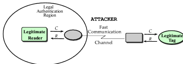
Fig. 1. Mafia and terrorist fraud scenarios
