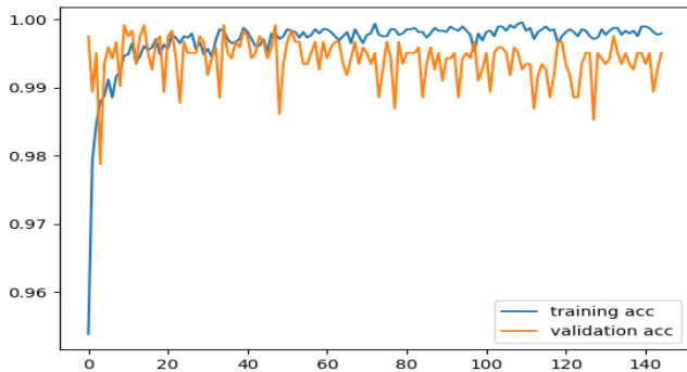
Figure 4: Training and validation accuracies at different epochs up to 145. These plots correspond to the training and validation losses depicted in Figure 3.
