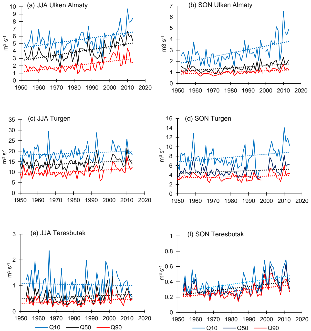
Figure 8. Time series of Q10, Q50 and Q90 flow thresholds with linear trends (dashed straight lines) for the Ulken Almaty, Turgen and Teresbutak for JJA and SON.
